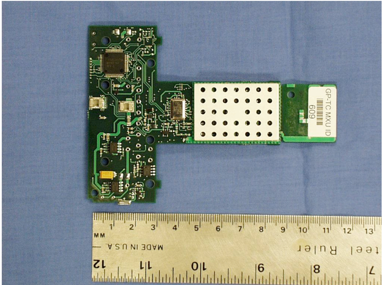
Top view
