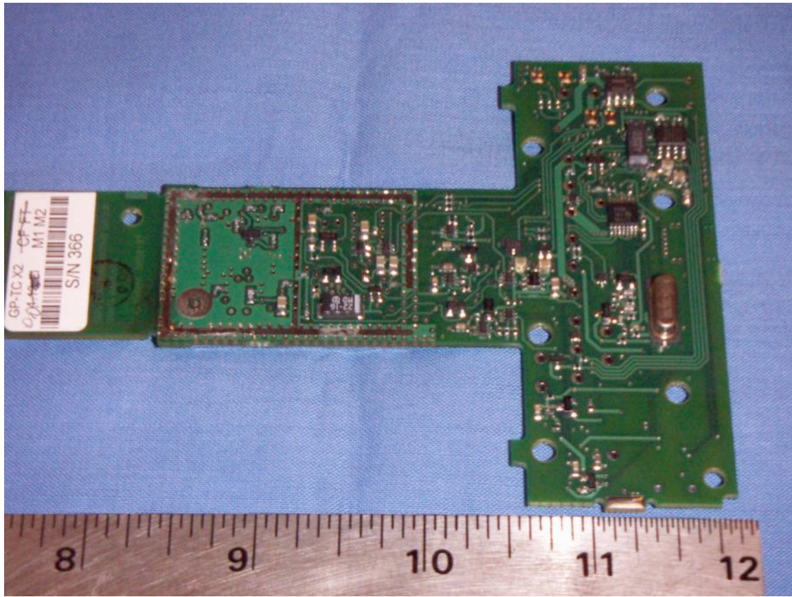
Bottom view
