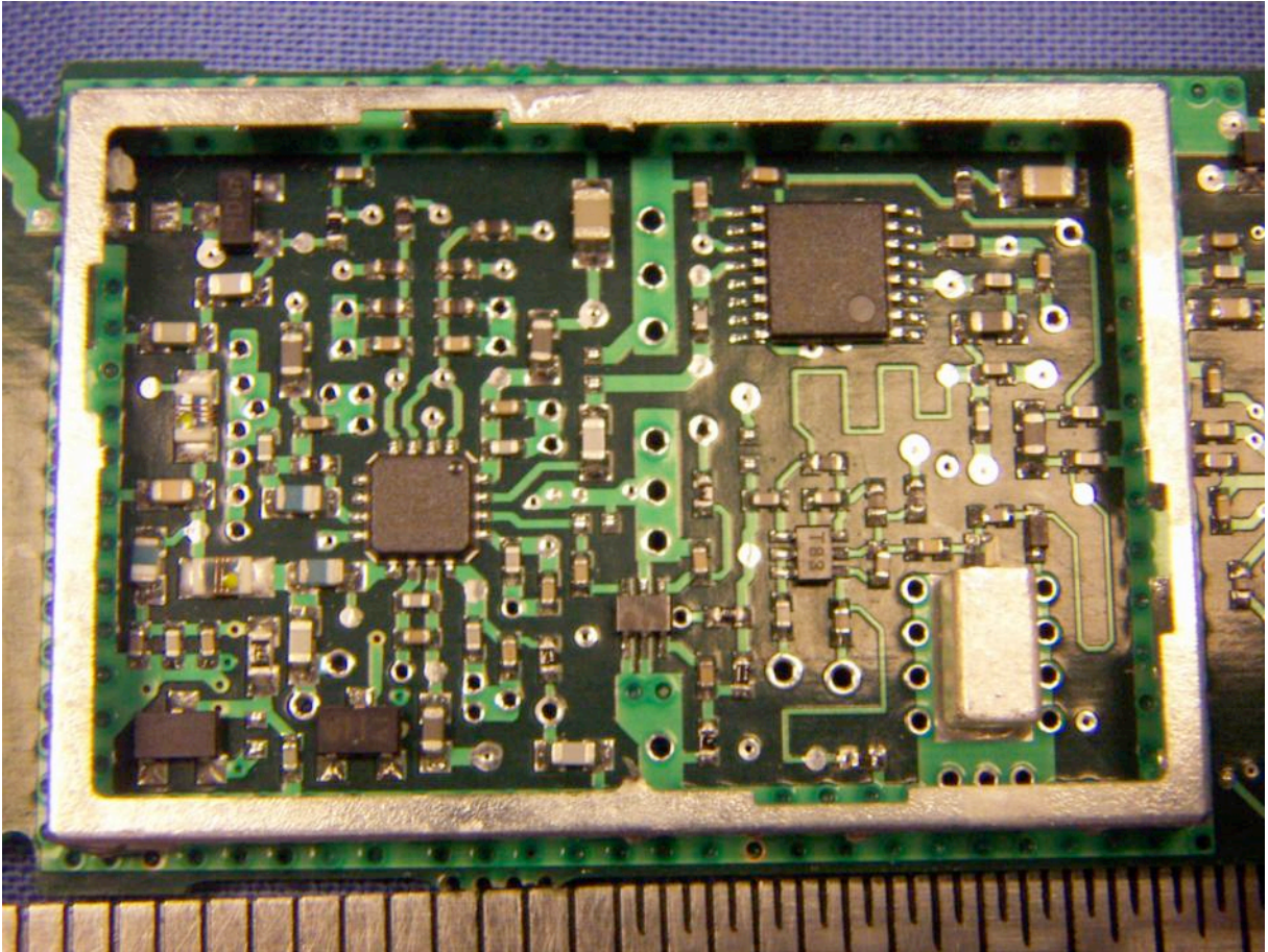
Under shield
