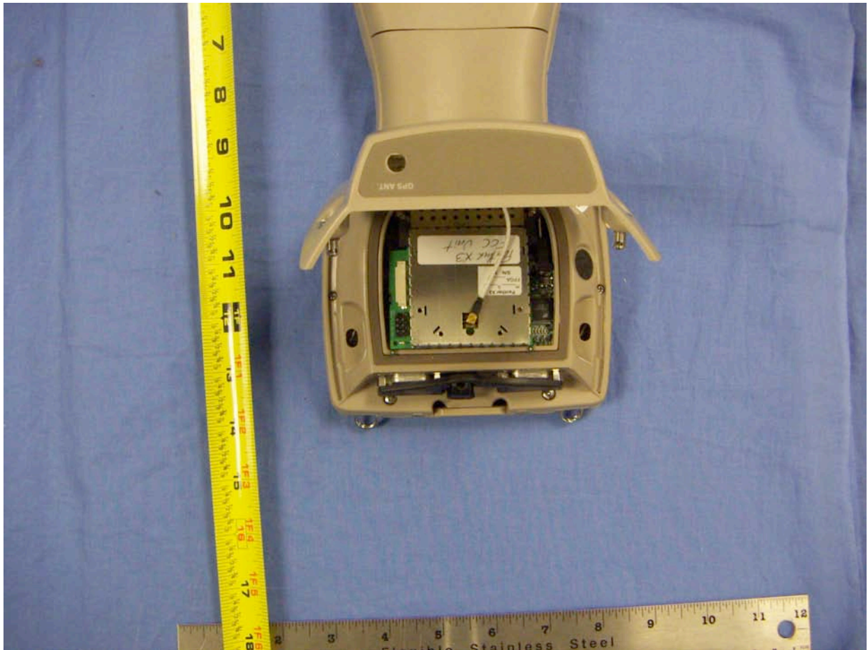
Location of RF module and antenna connector
