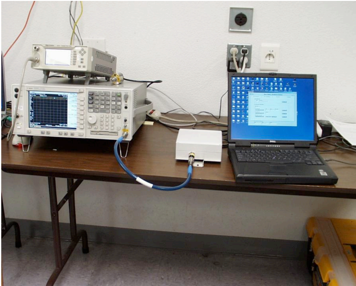
antenna port
