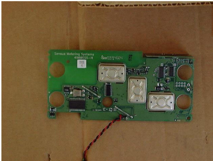
Figure 2 PCB Side 1
