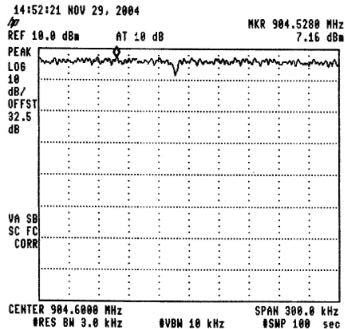
Figure 64 —904.6 MHz
