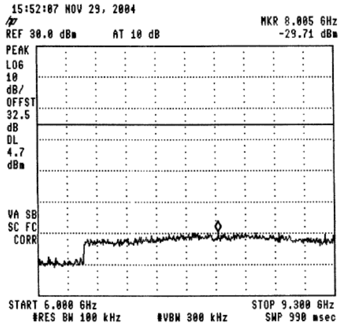
Figure 52 —925.4 MHz
