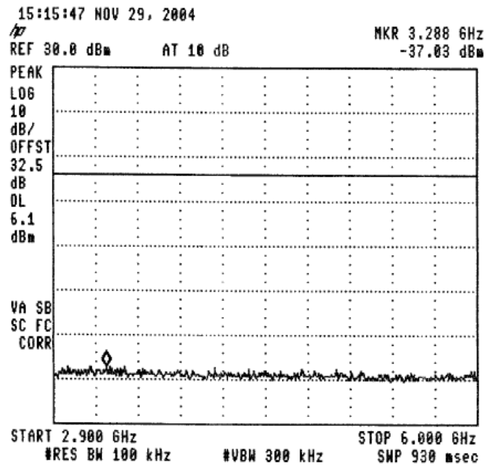
Figure 34 —904.6 MHz
