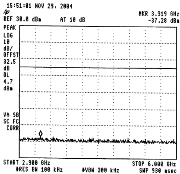
Figure 51 —925.4 MHz
