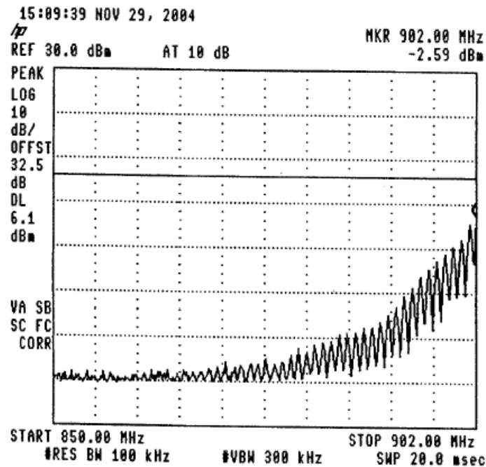
Figure 60 —904.6 MHz
