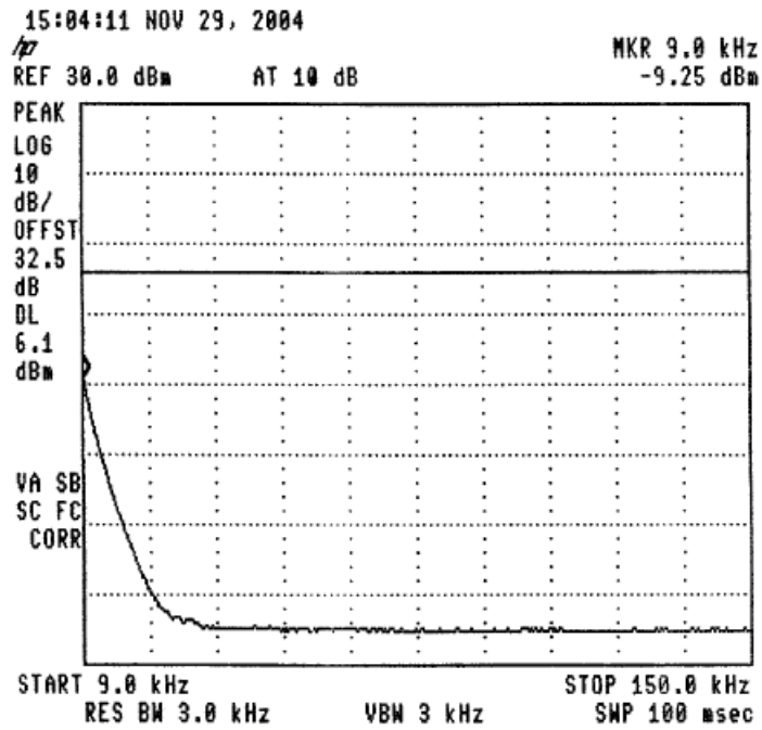
Figure 28 —904.6 MHz
