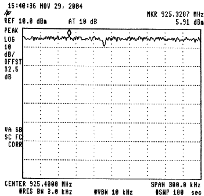
Figure 66 —925.4 MHz
