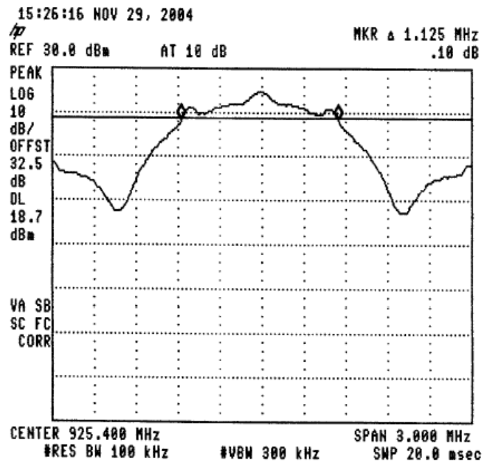
Figure 57 —925.4 MHz
