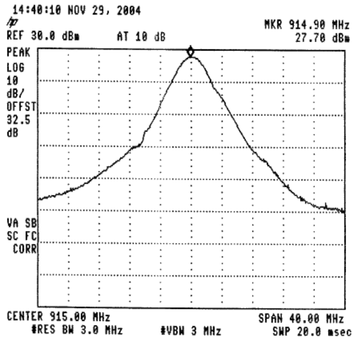
Figure 23 915.0 MHz
