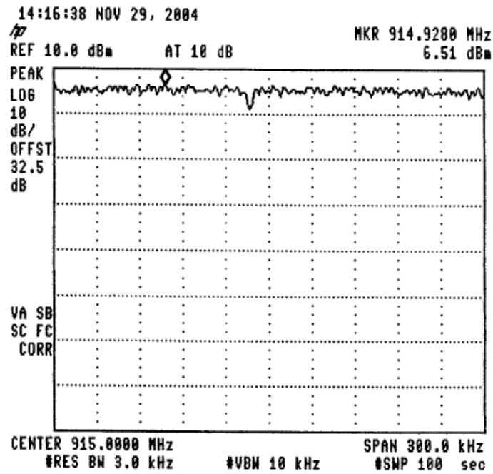
Figure 65 —915.0 MHz
