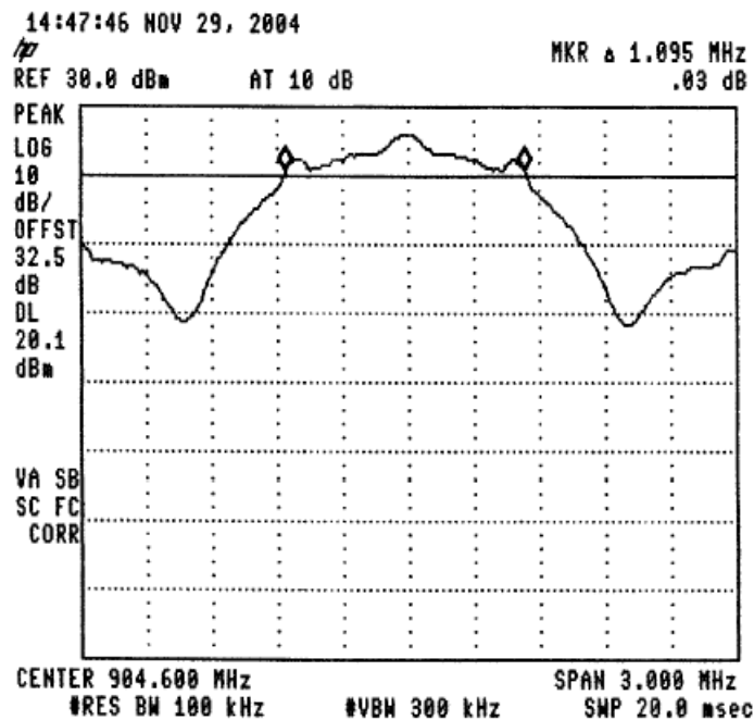
Figure 55 —904.6 MHz
