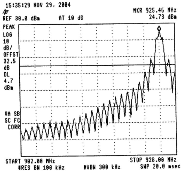
Figure 44 —925.4 MHz
