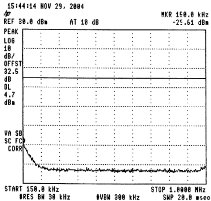
Figure 46 —925.4 MHz
