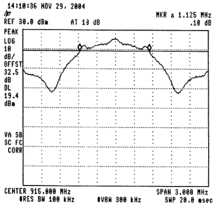
Figure 56 —915.0 MHz
