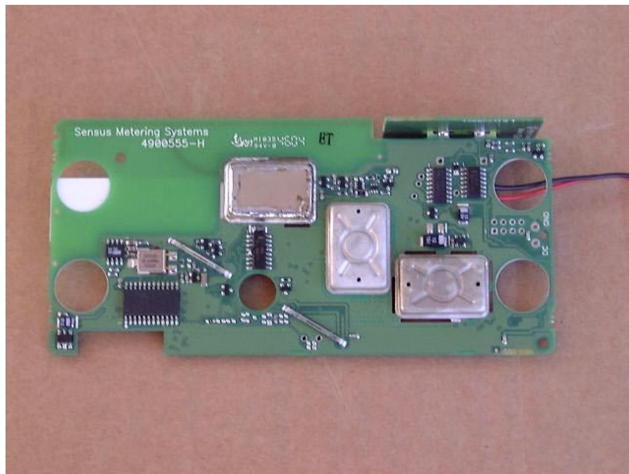
Figure 74 PCB Side 2
