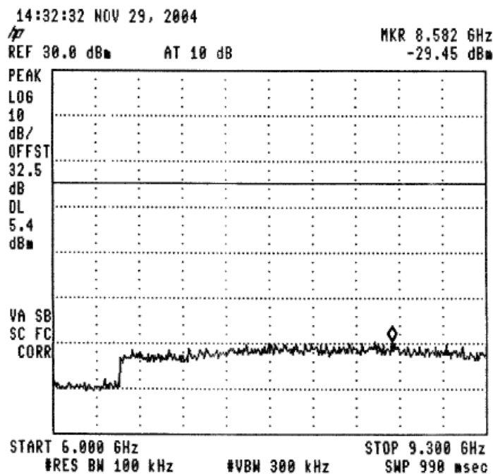
Figure 43 —915.0 MHz
