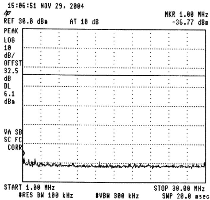
Figure 30 —904.6 MHz
