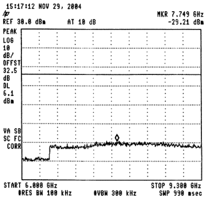
Figure 35 —904.6 MHz
