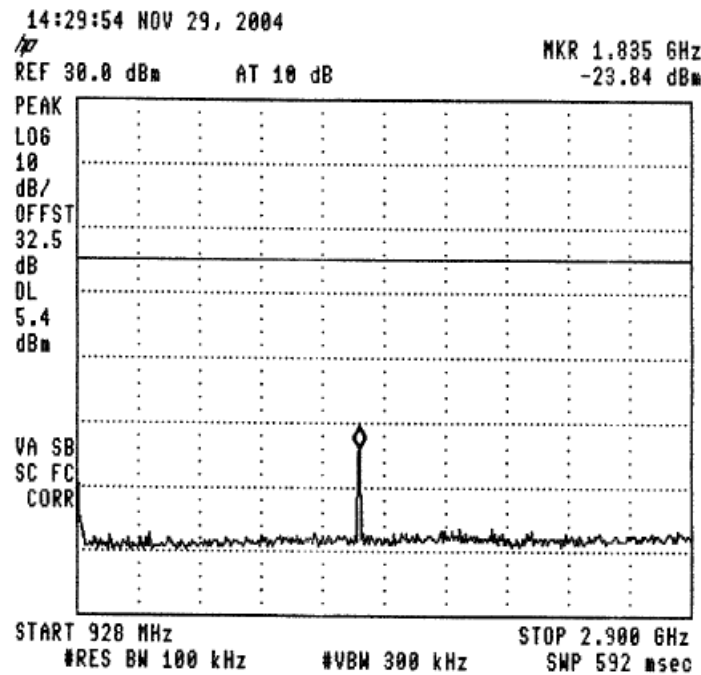
Figure 41 —915.0 MHz
