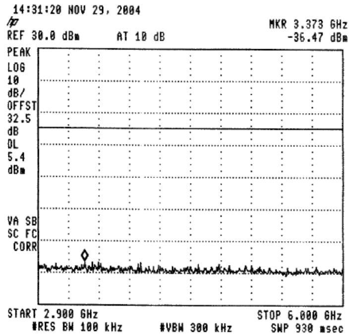
Figure 42 —915.0 MHz
