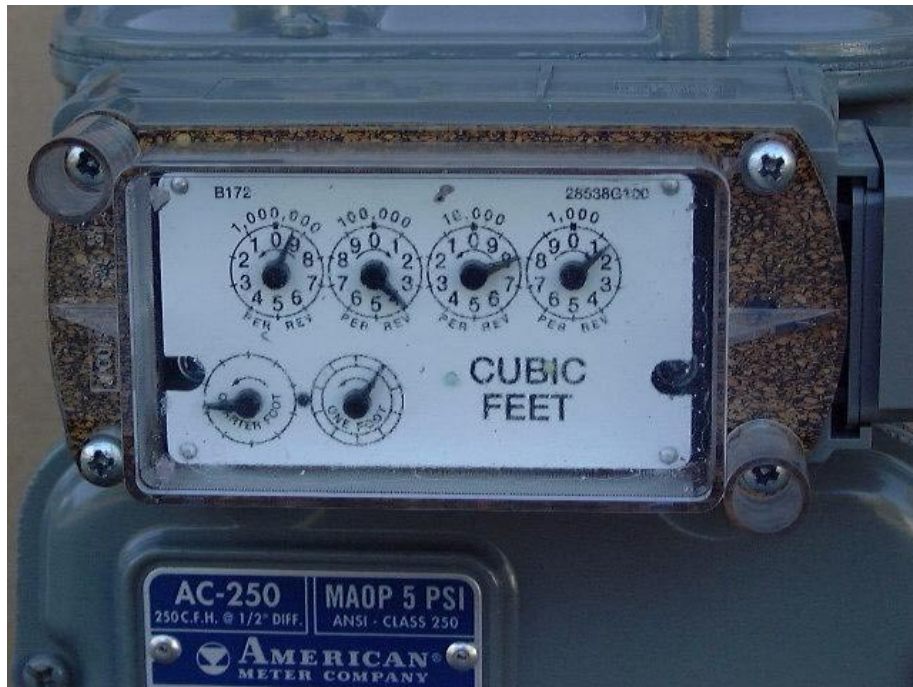
Figure 69 Front View With Cover
