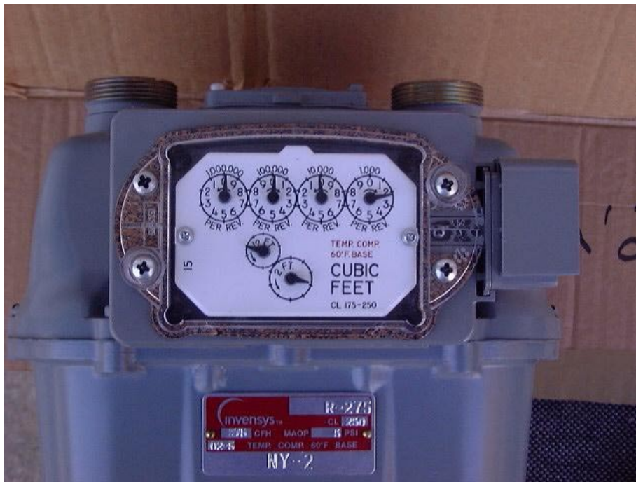
Figure 1 Front Panel With Cover
