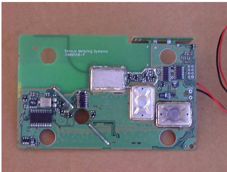
Figure 4 PCB Side 2
