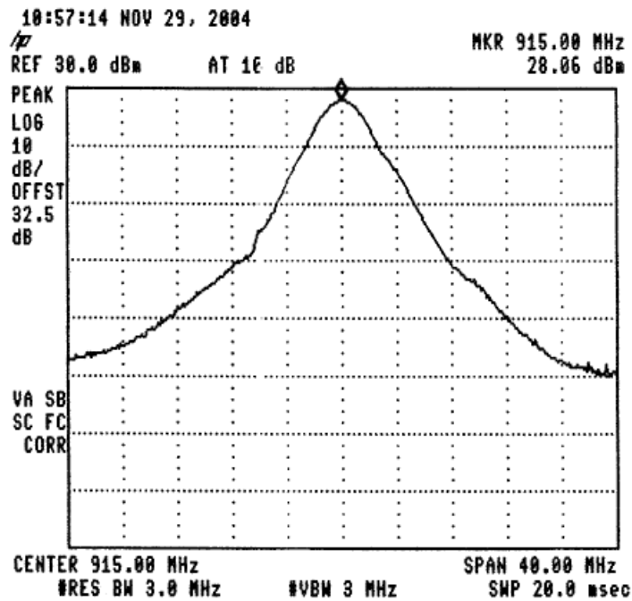
Figure 23 915.0 MHz
