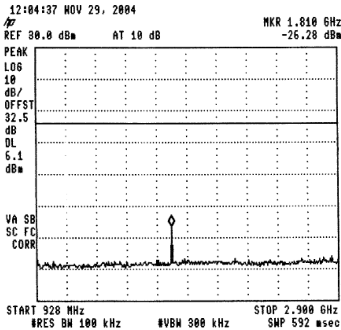
Figure 33 —904.6 MHz
