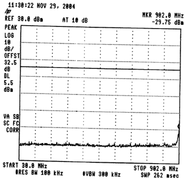
Figure 40 —915.0 MHz
