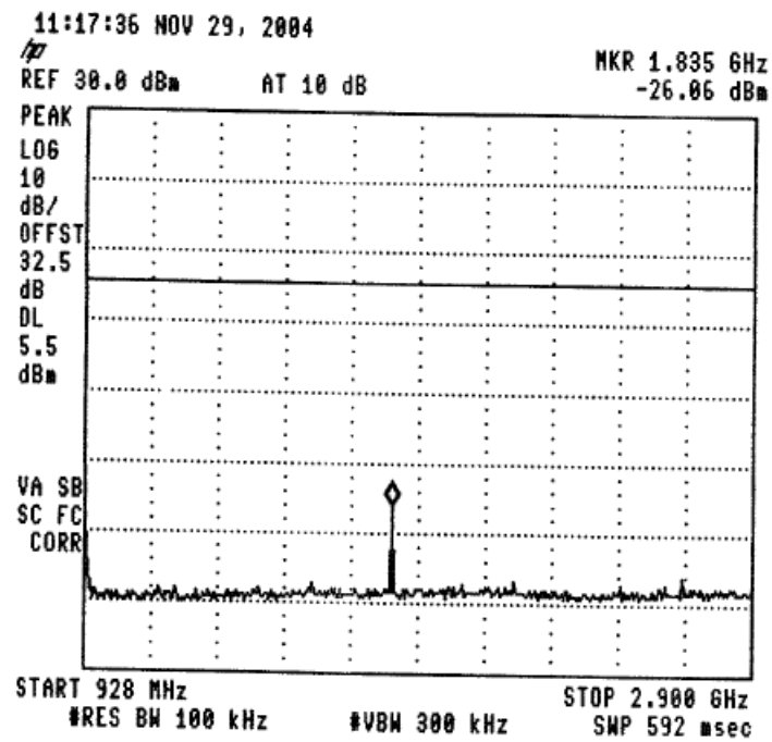
Figure 41 —915.0 MHz
