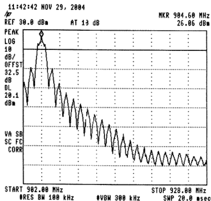
Figure 27 —904.6 MHz
