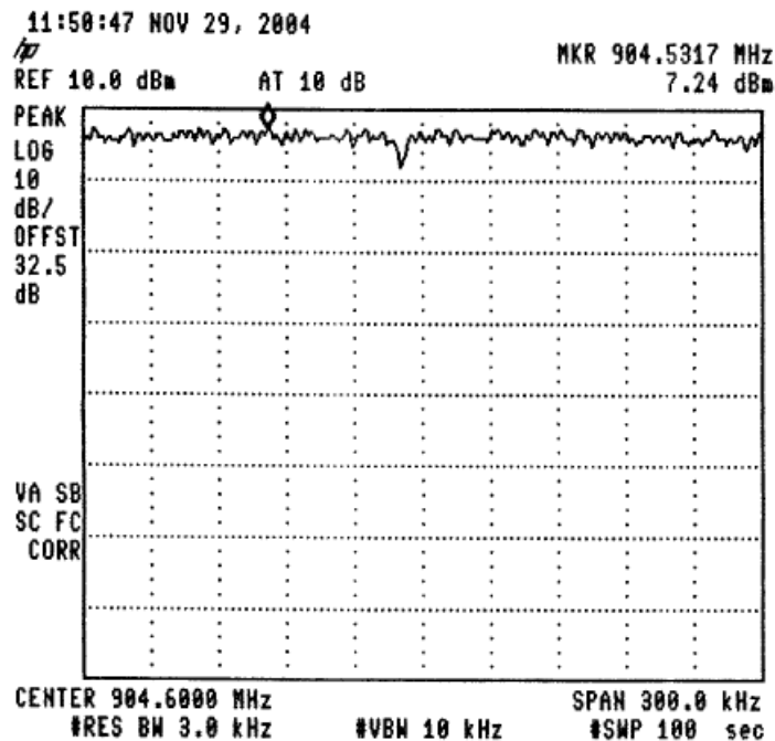
Figure 64 —904.6 MHz
