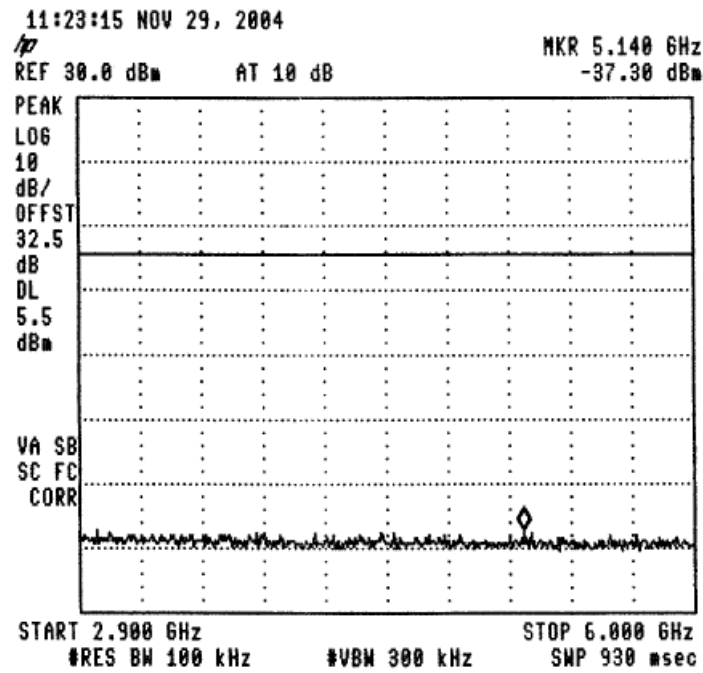
Figure 42 —915.0 MHz
