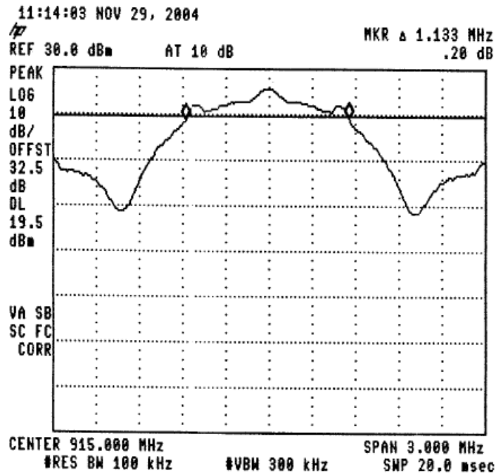
Figure 56 —915.0 MHz
