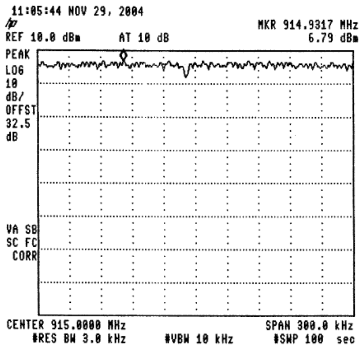
Figure 65 —915.0 MHz
