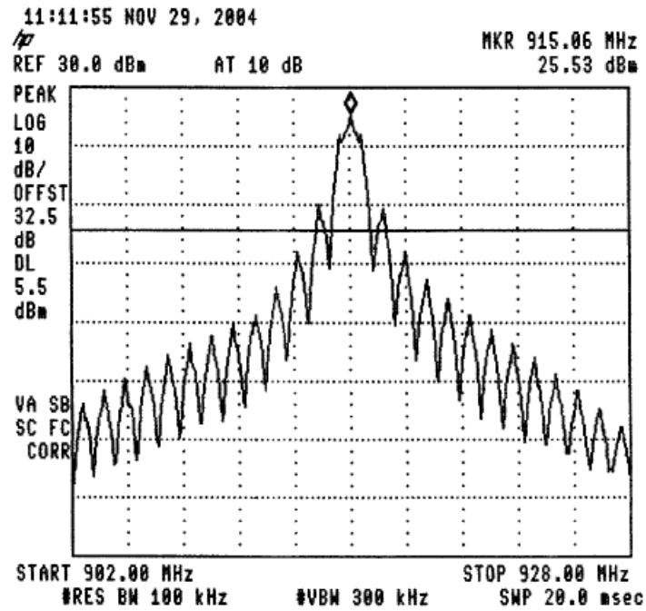
Figure 36 —915.0 MHz
