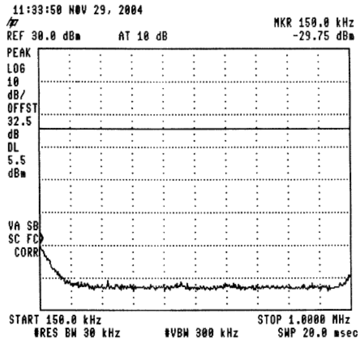
Figure 38 —915.0 MHz
