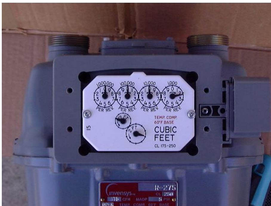
Figure 70 Front Panel Without Cover
