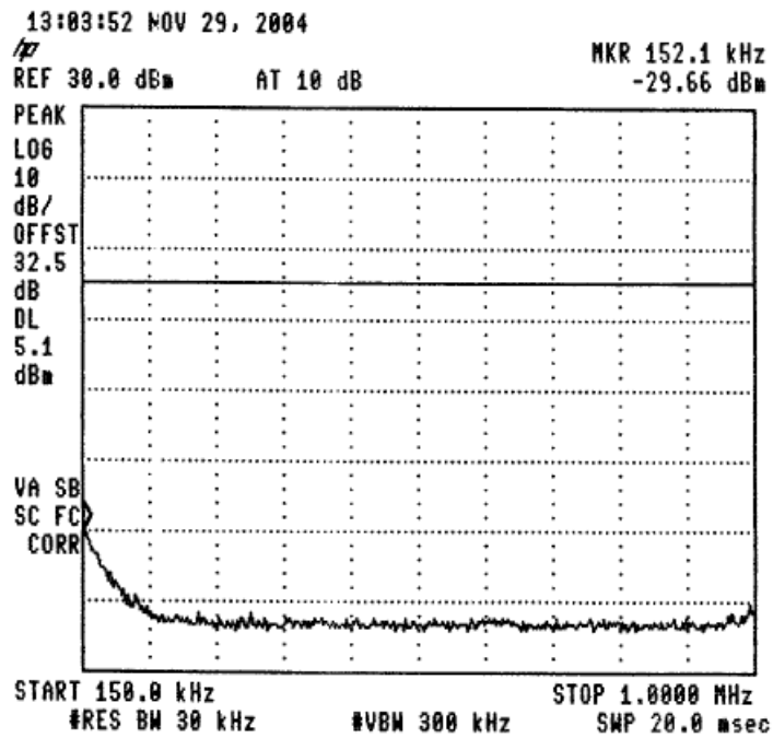
Figure 46 —925.4 MHz
