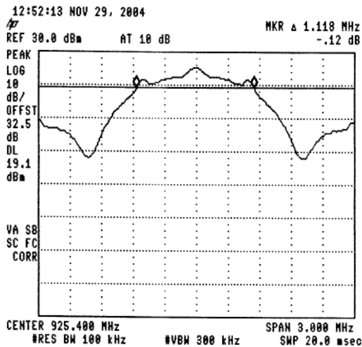
Figure 57 —925.4 MHz
