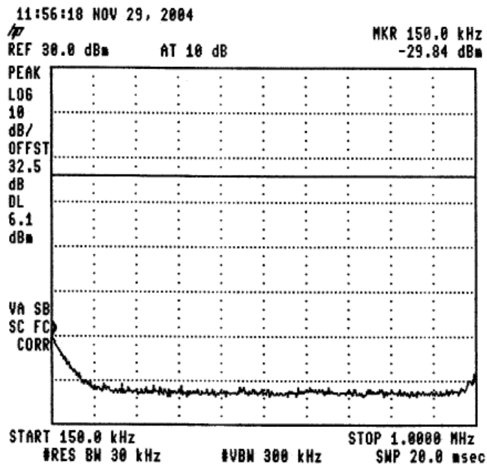
Figure 29 —904.6 MHz
