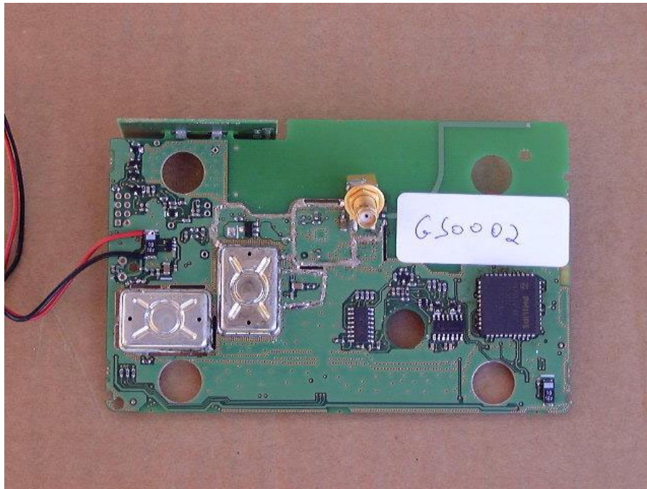
Figure 73 PCB Side 1
