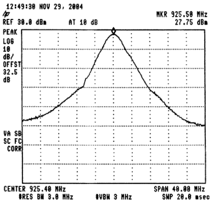
Figure 24 925.4 MHz
