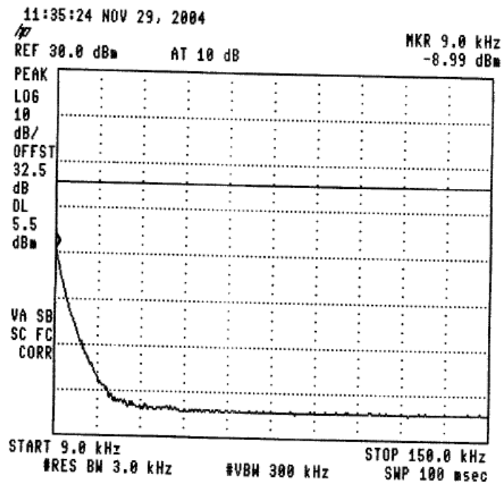
Figure 37 —915.0 MHz
