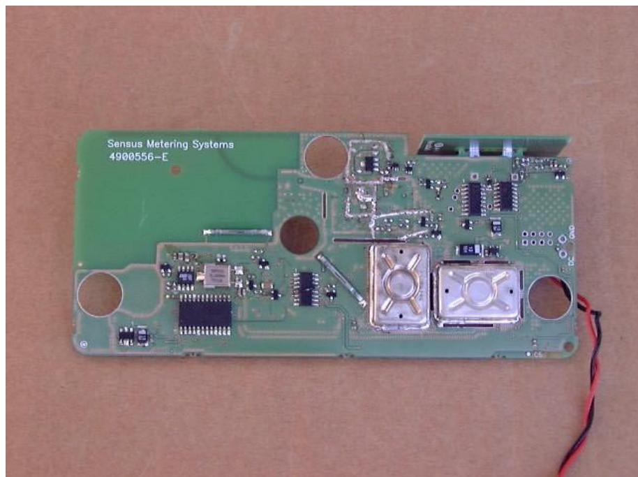
Figure 2 PCB Side 2
