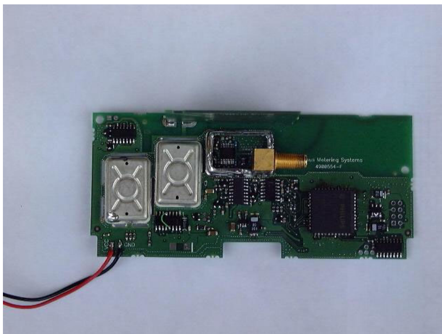
Figure 1 PCB Side 1
