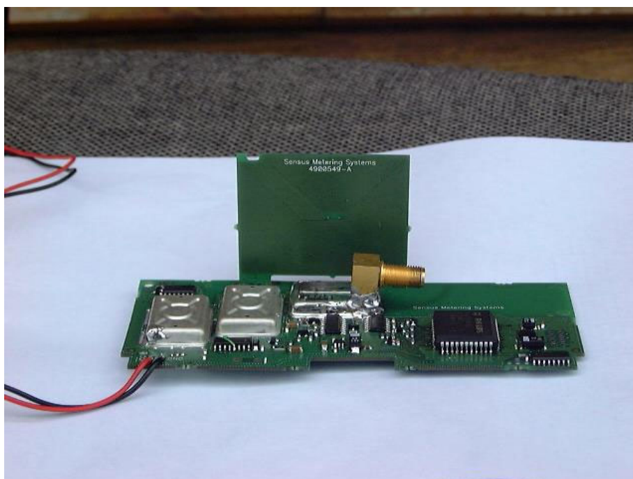
Figure 2 PCB Side 1
