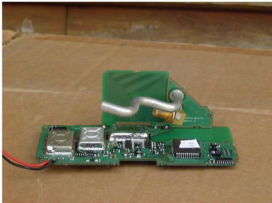
Figure 4 PCB Side 1
