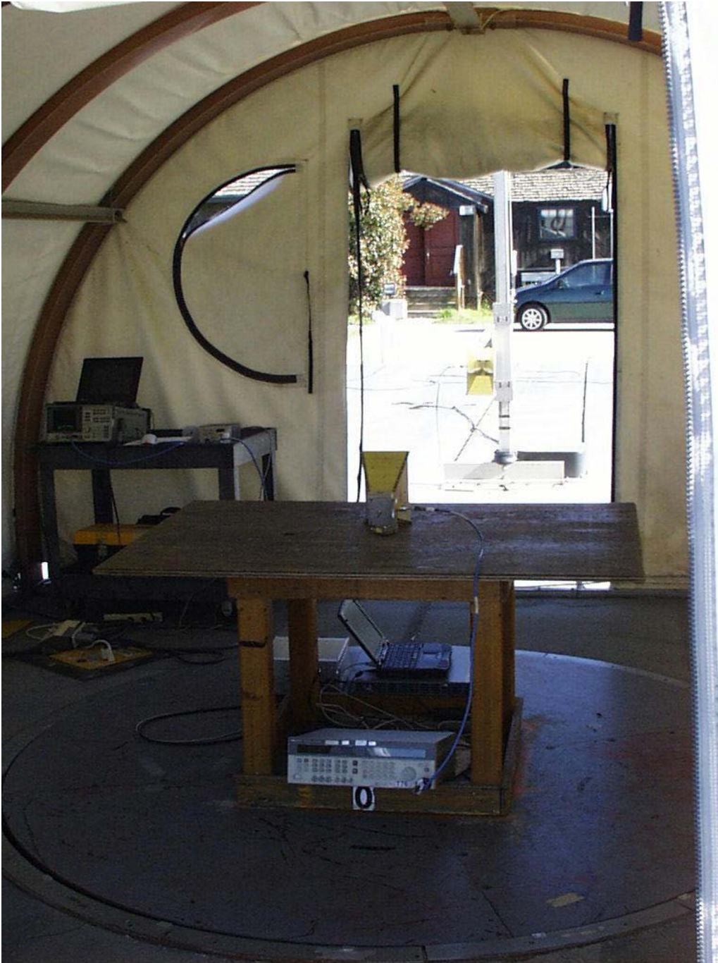
Substitution test set-up, 1-18 GHz
