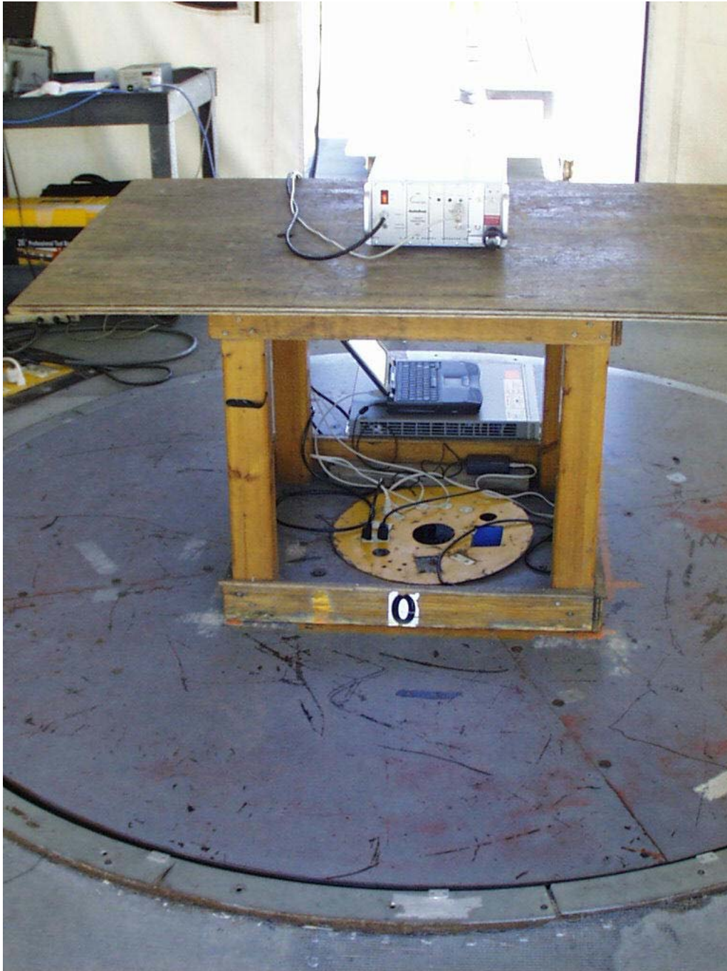
Radiated emissions, substitution method, equipment front view
