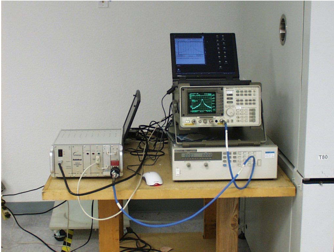
Antenna conducted set-up
