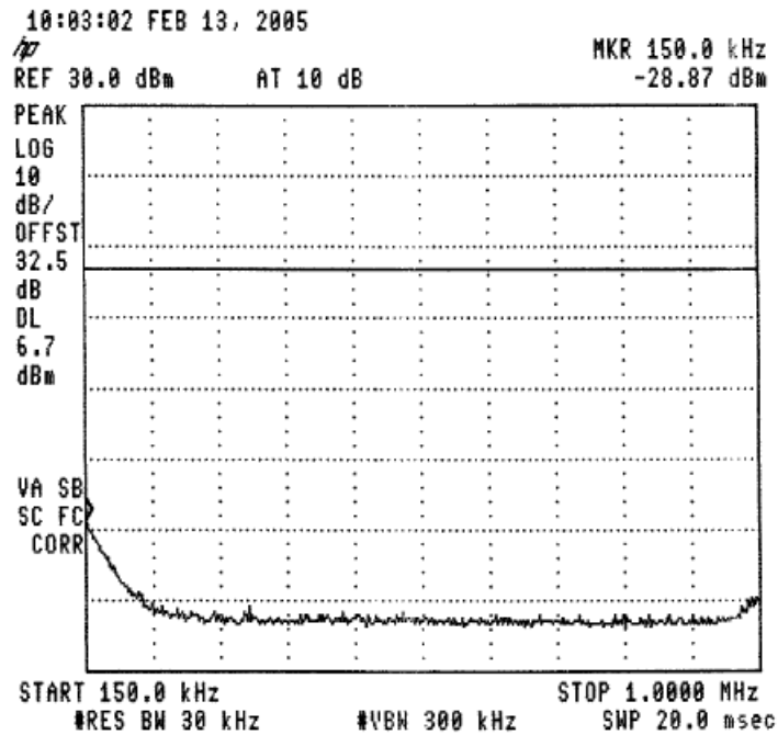
Figure 40 —915.0 MHz
