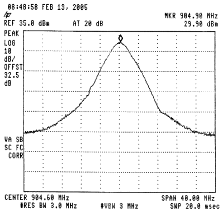
Figure 24 904.6 MHz
