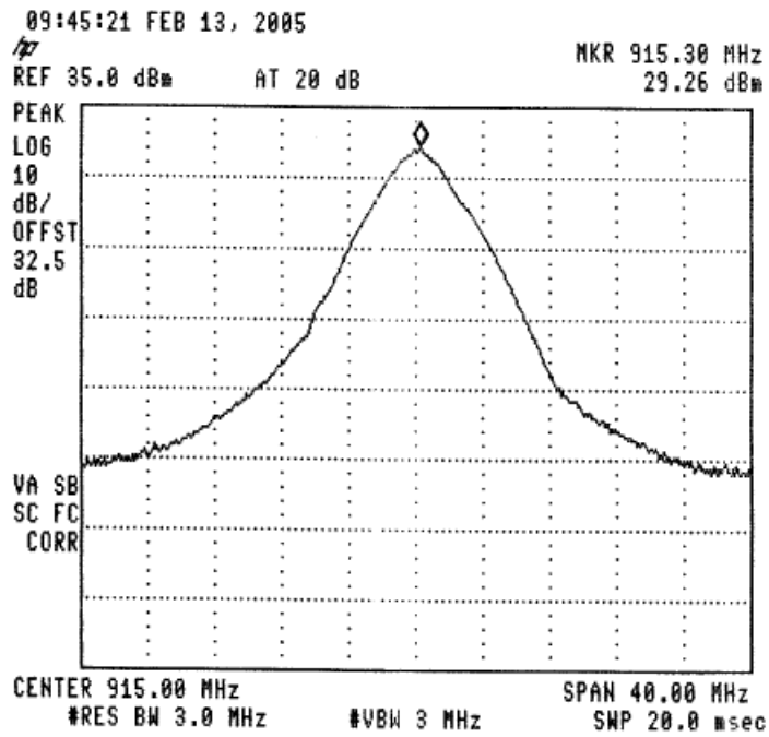
Figure 25 915.0 MHz
