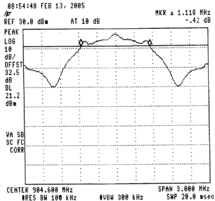
Figure 57 —904.6 MHz
