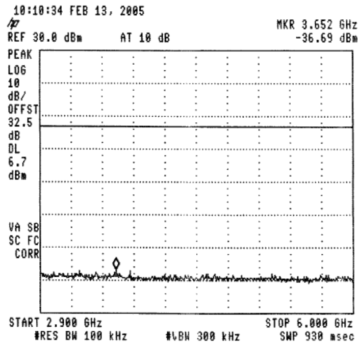
Figure 44 —915.0 MHz
