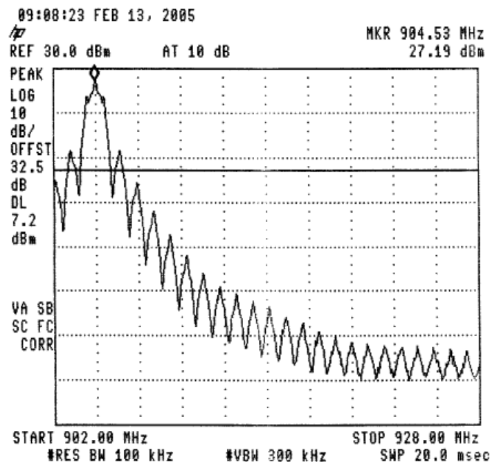
Figure 29 —904.6 MHz
