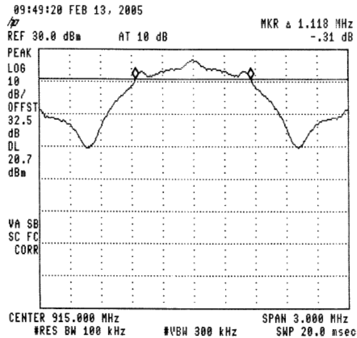
Figure 58 —915.0 MHz
