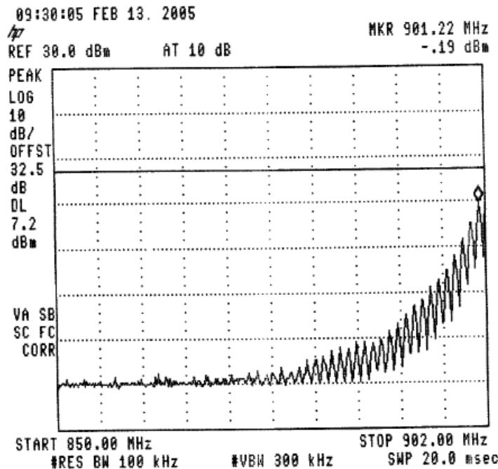
Figure 62 —904.6 MHz
