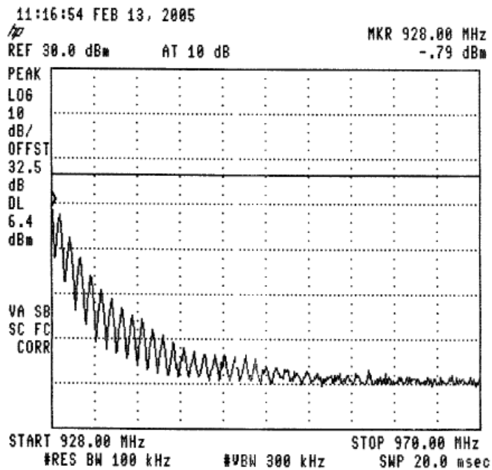
Figure 51 —925.4 MHz
