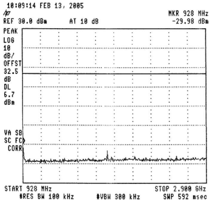
Figure 43 —915.0 MHz
