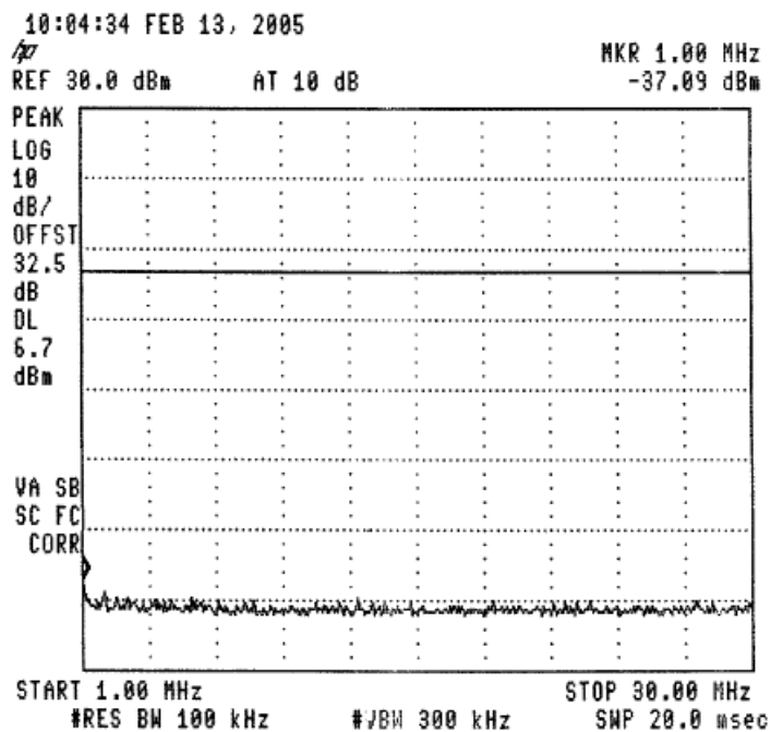
Figure 41 —915.0 MHz
