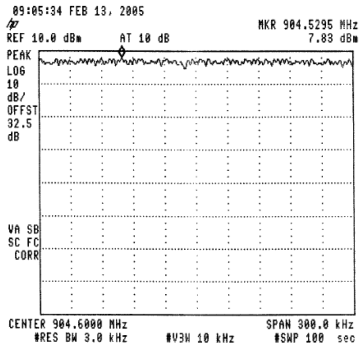
Figure 66 —904.6 MHz
