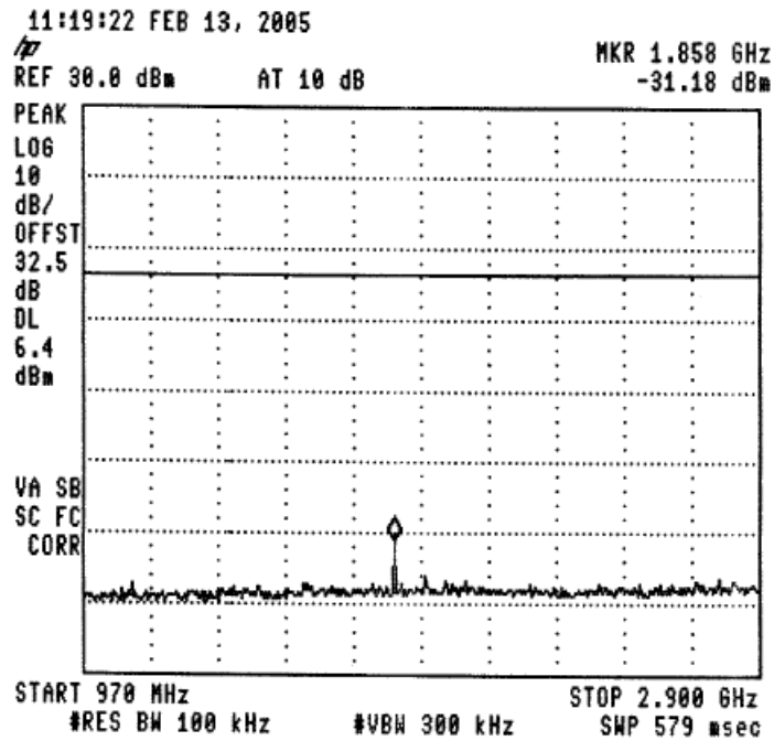
Figure 52 —925.4 MHz
