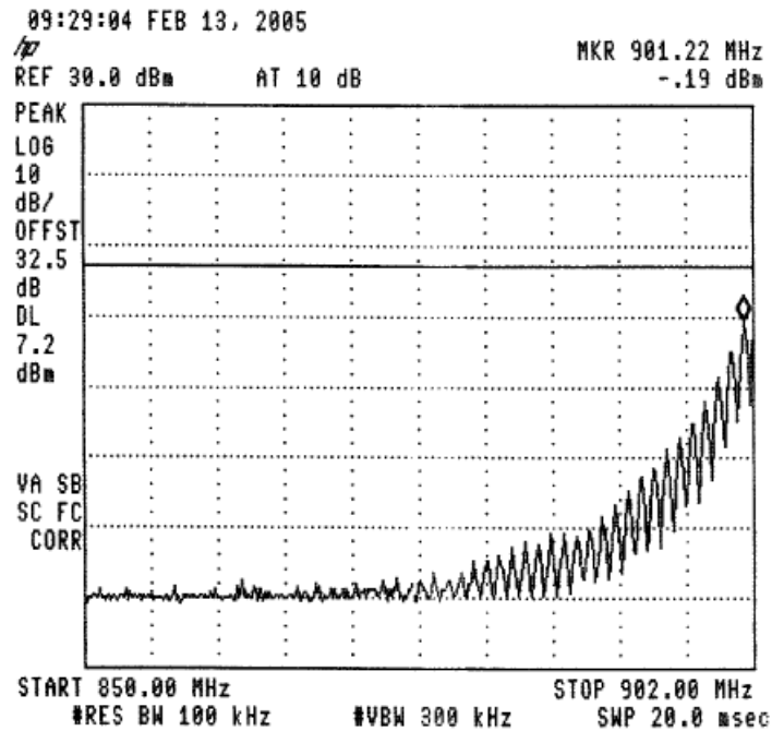
Figure 34 —904.6 MHz
