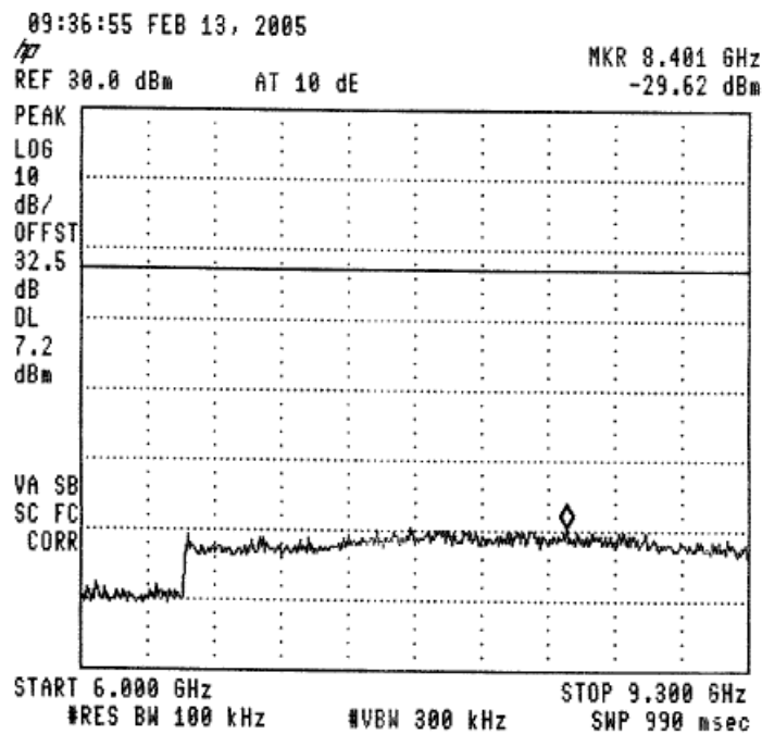
Figure 37 —904.6 MHz
