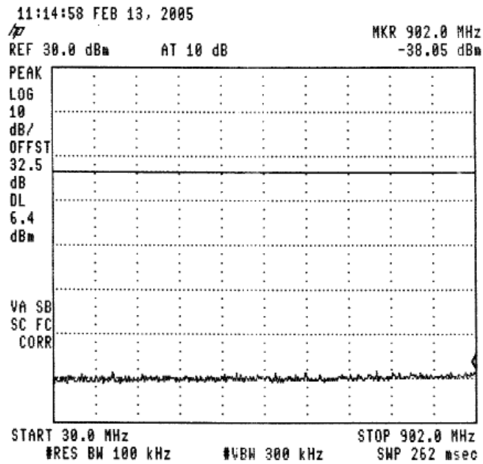
Figure 50 —925.4 MHz
