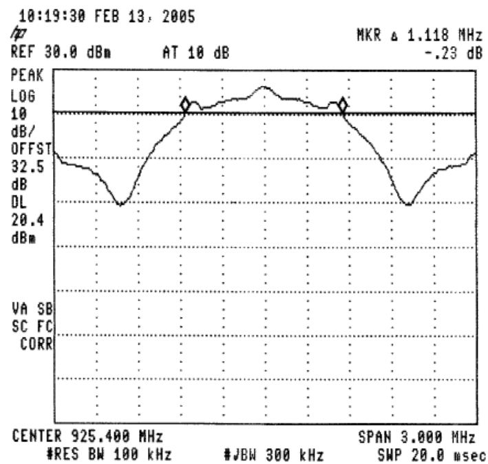
Figure 59 —925.4 MHz
