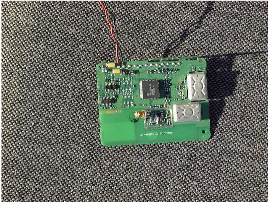
Figure 75 PCB Side 1
