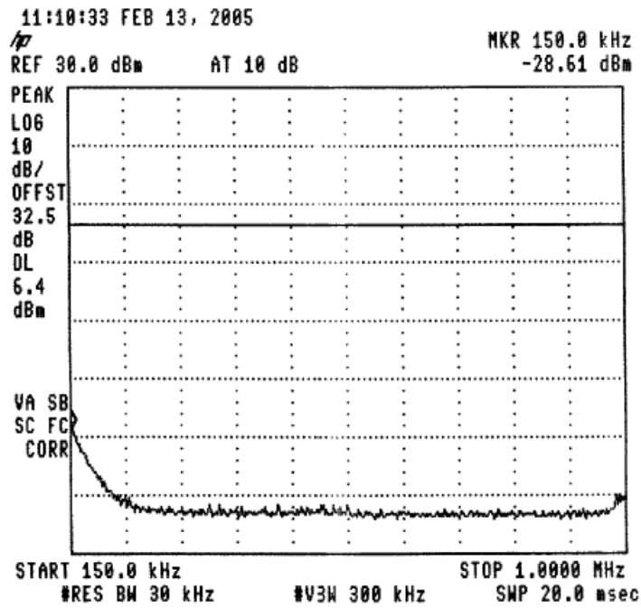
Figure 48 —925.4 MHz
