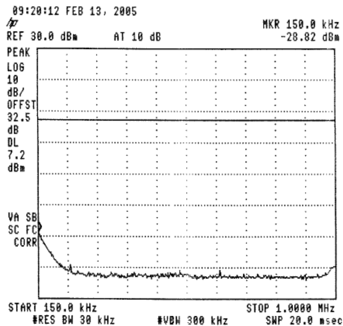
Figure 31 —904.6 MHz
