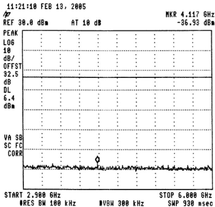
Figure 53 —925.4 MHz
