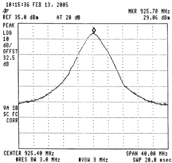
Figure 26 925.4 MHz
