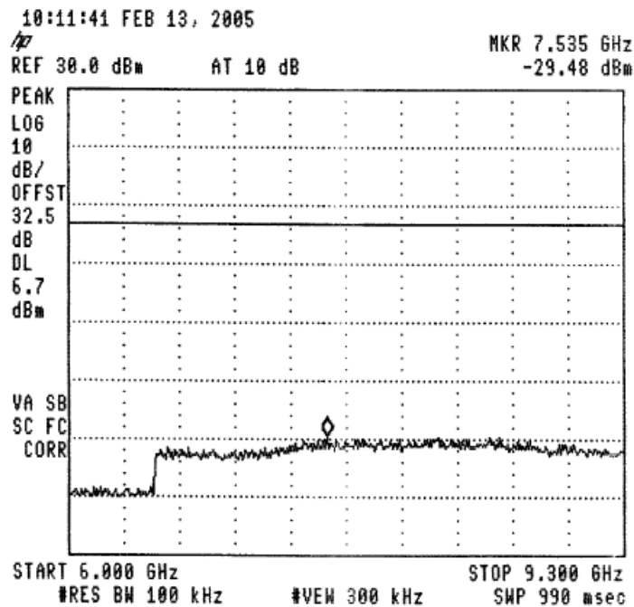
Figure 45 —915.0 MHz
