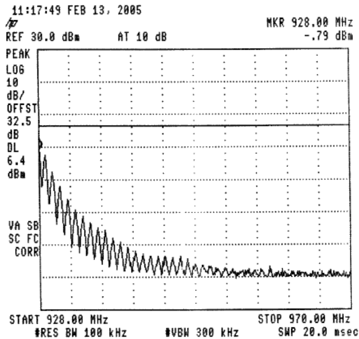
Figure 63 —925.4 MHz
