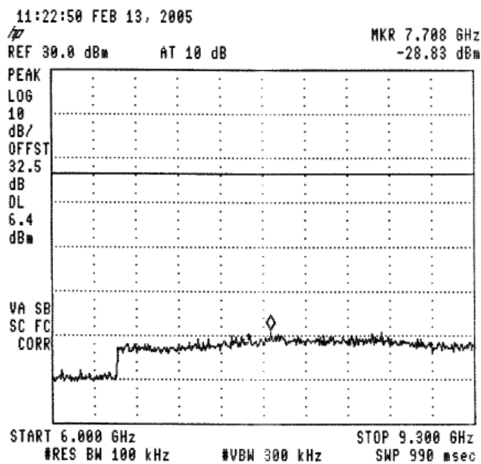
Figure 54 —925.4 MHz
