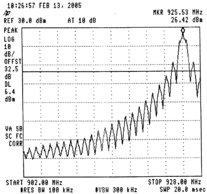
Figure 46 —925.4 MHz
