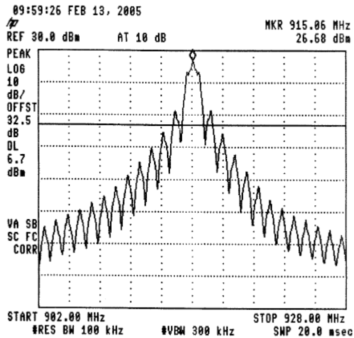
Figure 38 —915.0 MHz
