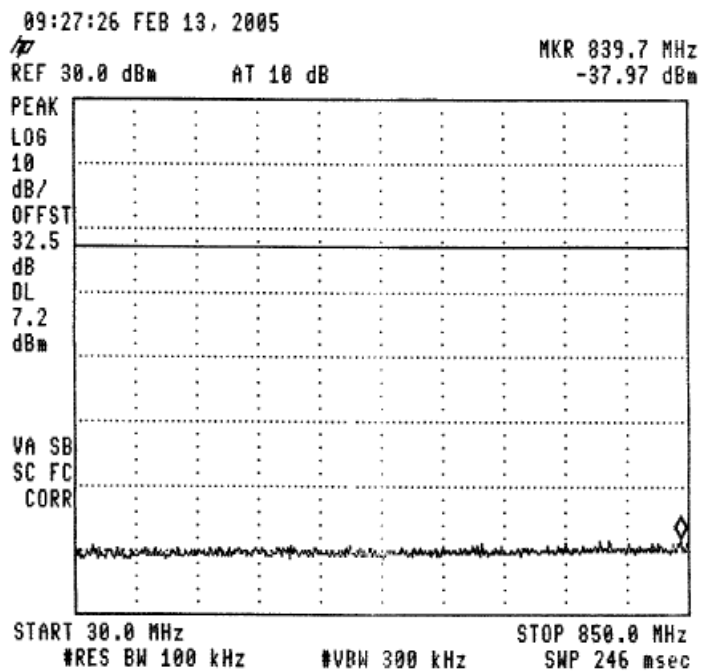
Figure 33 —904.6 MHz
