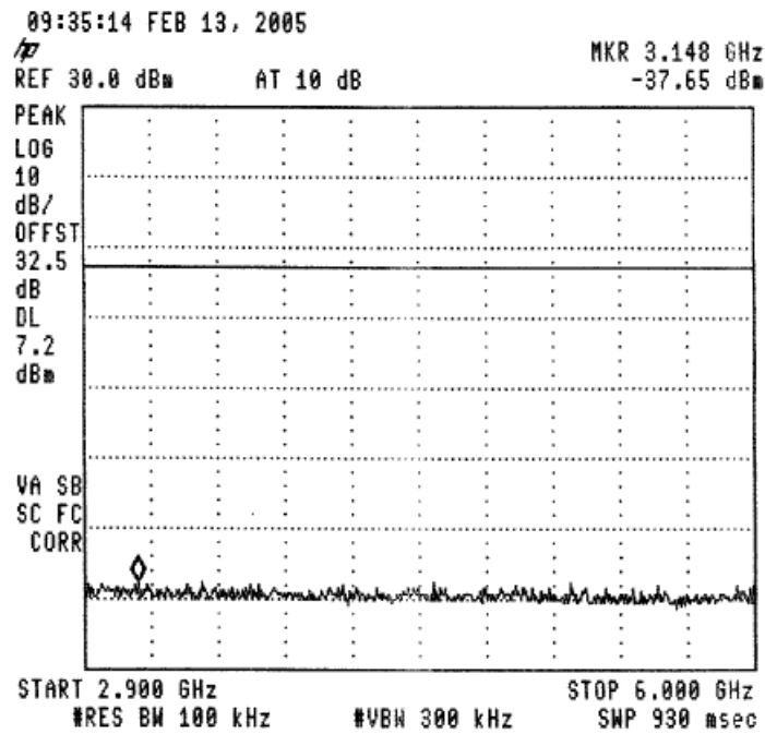
Figure 36 —904.6 MHz
