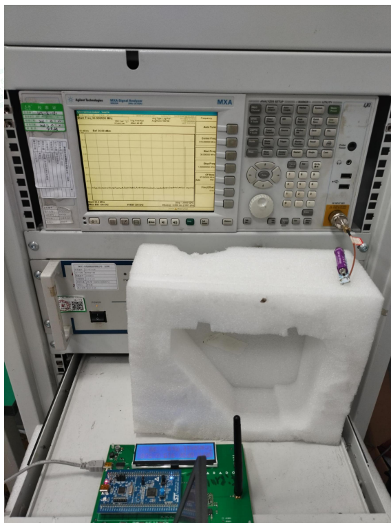
Fig. 3 RF conducted Measurement
