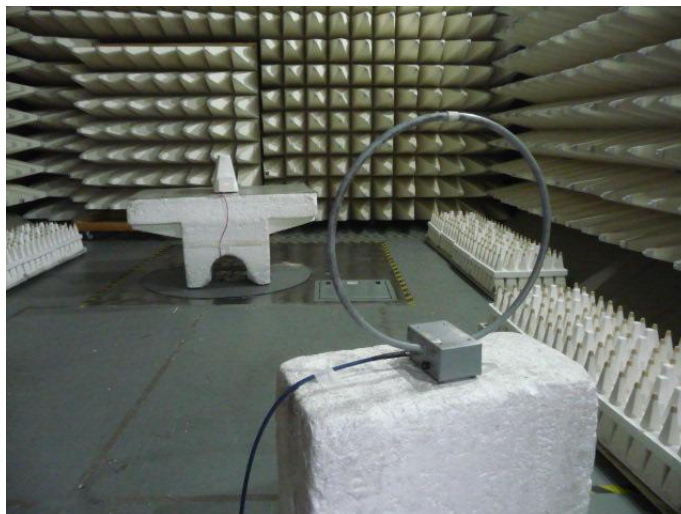
Photograph No.1 Setup for spurious field strength measurements in anechoic chamber from 9 kHz to 30 MHz
