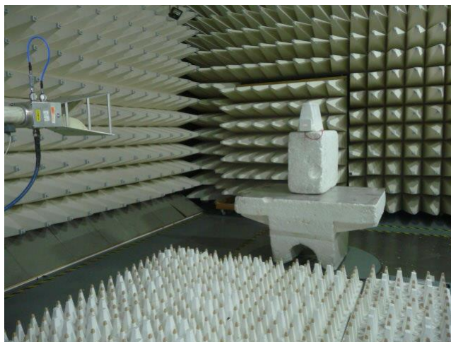
Photograph No.3 Setup for field strength measurements in anechoic chamber above 1 GHz
