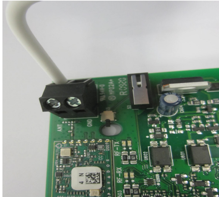
Photograph No.5 Antenna close view
