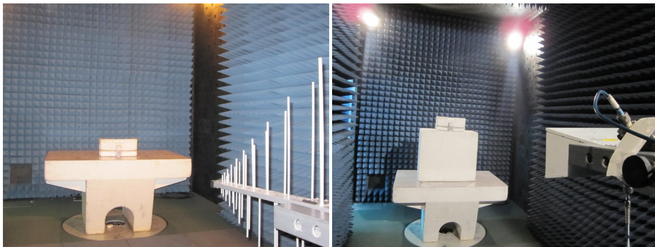
Photograph 8.1.2 Setup for final radiated emission measurements, EUT close view
