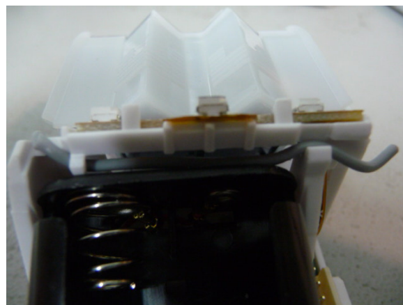
Photograph 7.4.1 Antenna assembly
