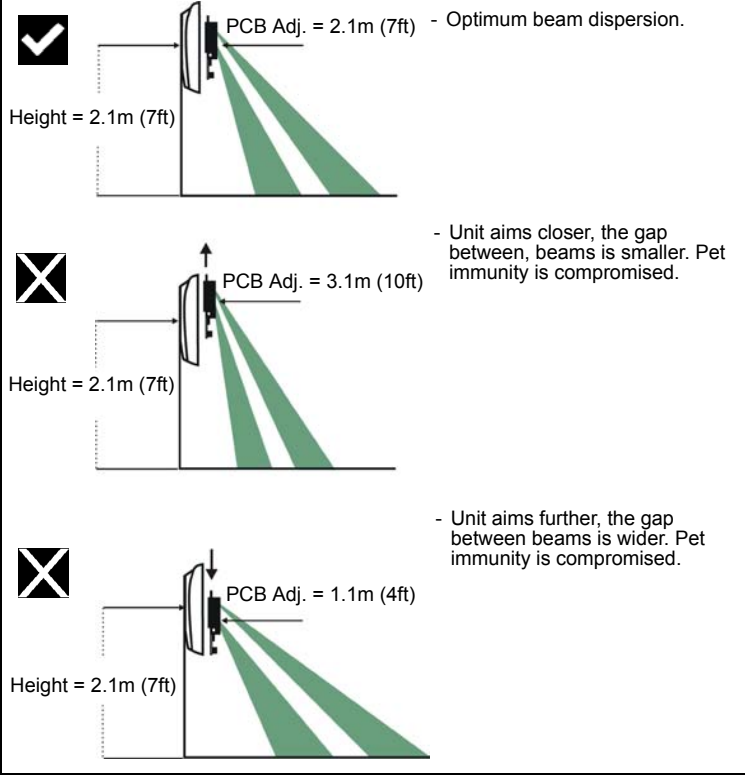
Figure 4 : PCB Settings
