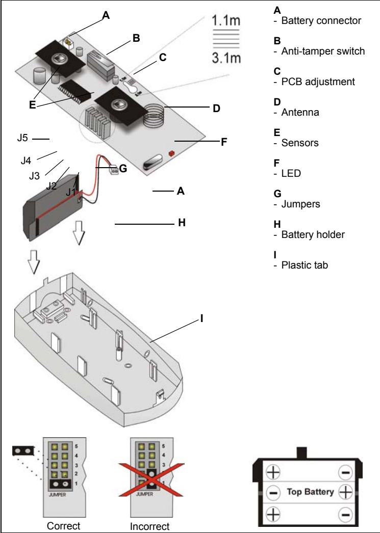
Figure 4 : PCB Settings
