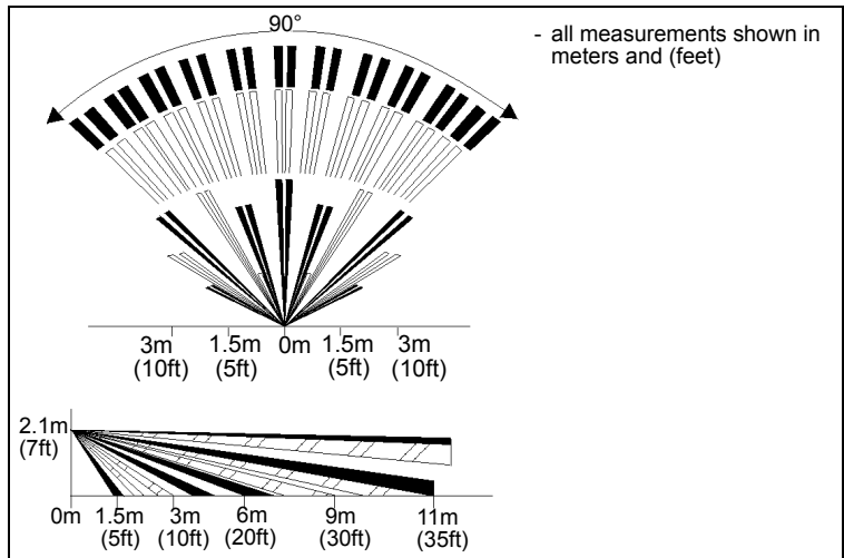
Figure 2 : Beam Dispersion
