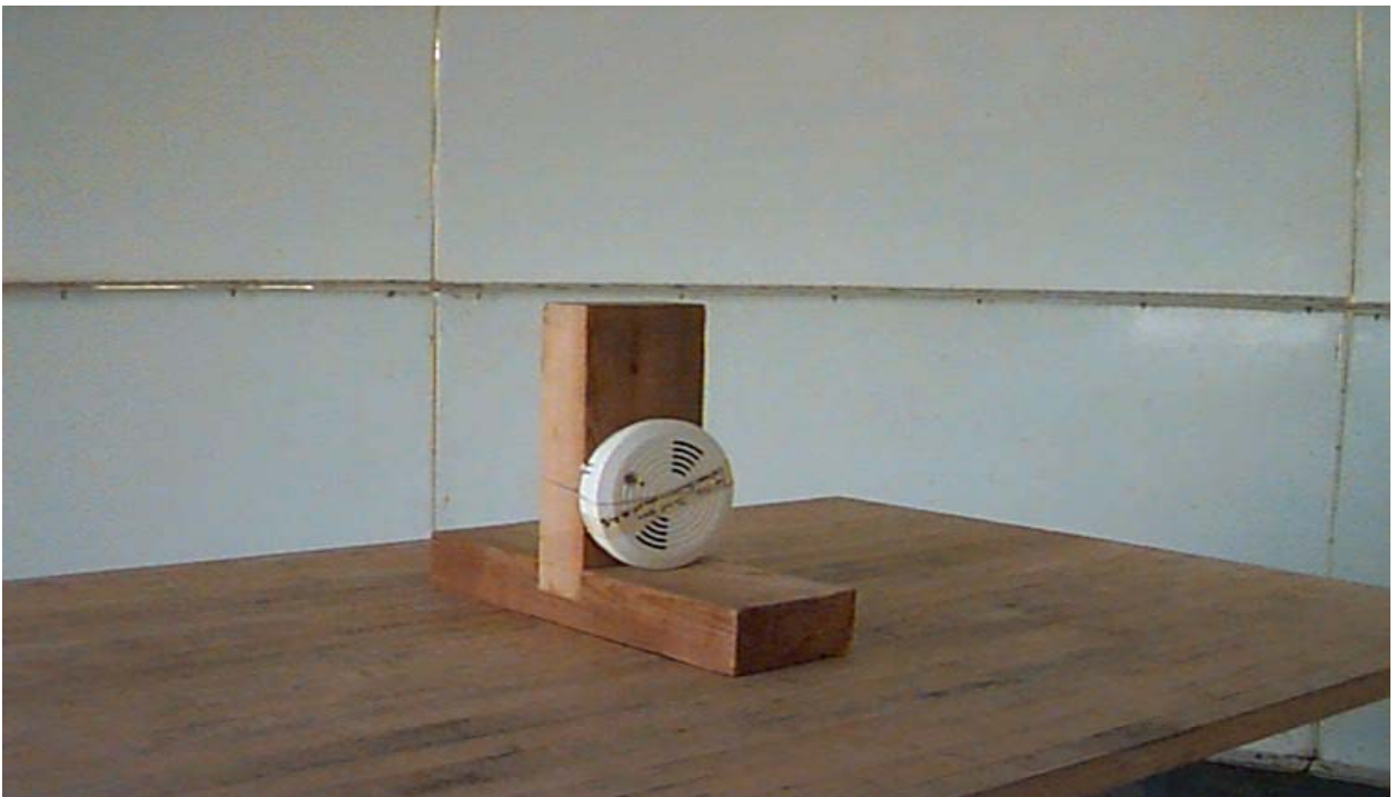
OATS Set Up Photo– FCC ID: KDYOMNSMK1
