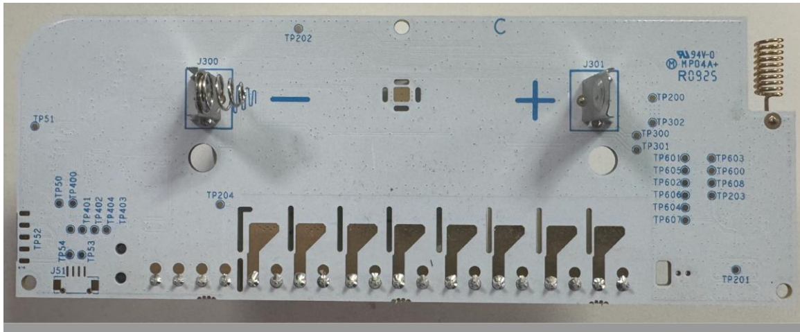
Photograph No.3 PGM8M Rear side of the main PCB
