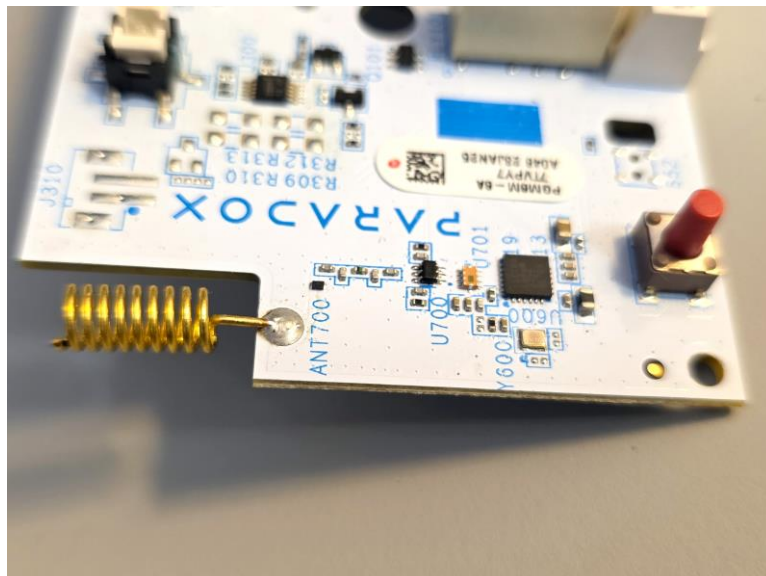
Photograph No.4 PGM8M Antenna assembly
