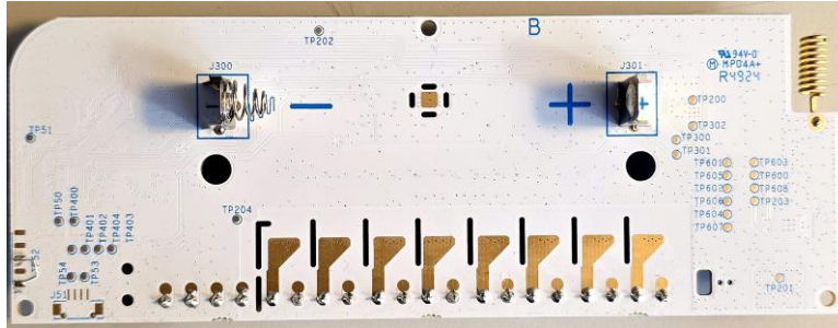
Photograph No.1 PGM8M Front side of the main PCB
