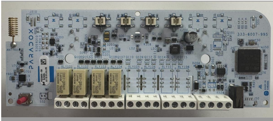
Photograph No.2 PGM4M Front side of the main PCB
