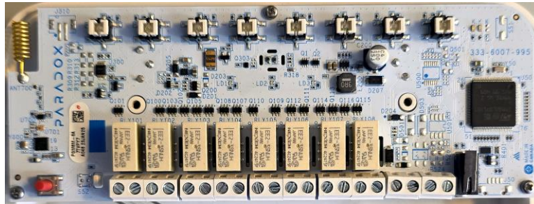
Photograph No.3 PGM8M Rear side of the main PCB
