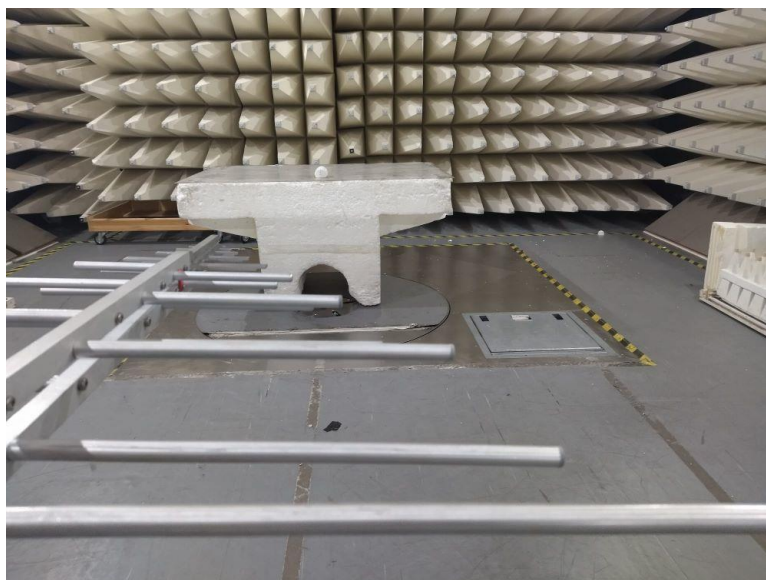
Photograph No.2 Setup for carrier and spurious emissions measurements in anechoic chamber from 30 MHz to 1 GHz
