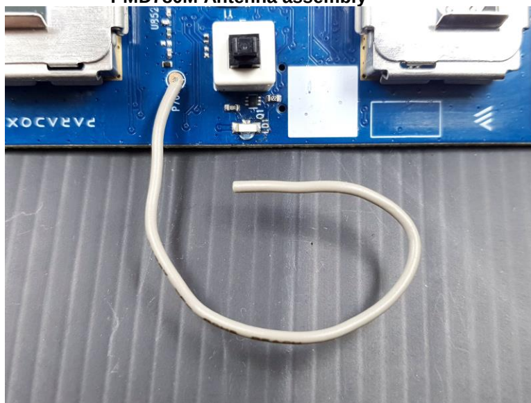
Photograph No.4 PMD780M Antenna assembly
