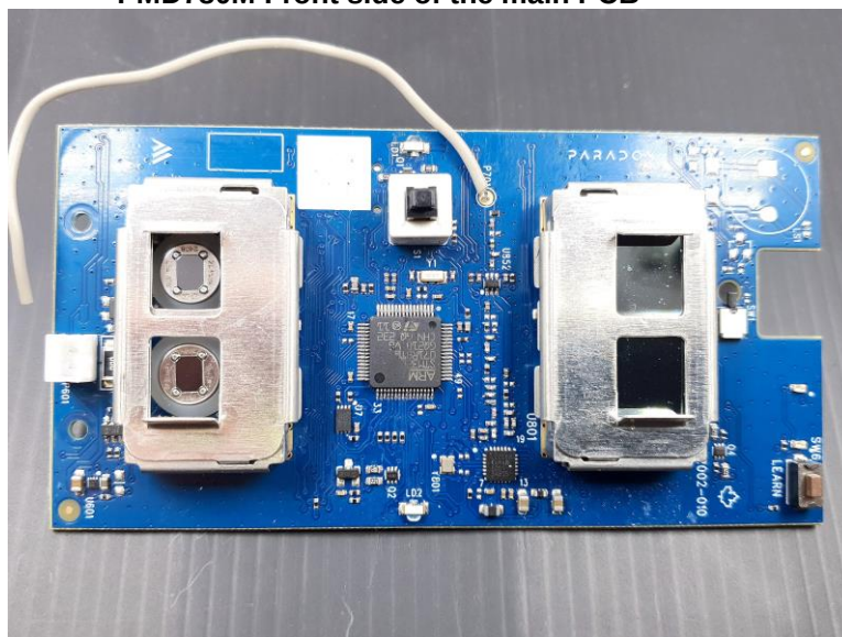
Photograph No.1 PMD780M Front side of the main PCB
