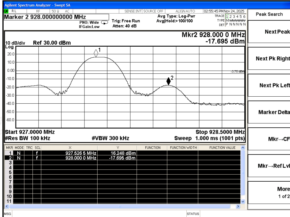
Ant1_High_927.55
