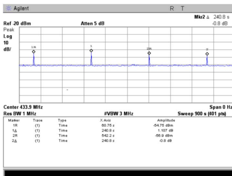
Plot 7.2.9 Transmission period
