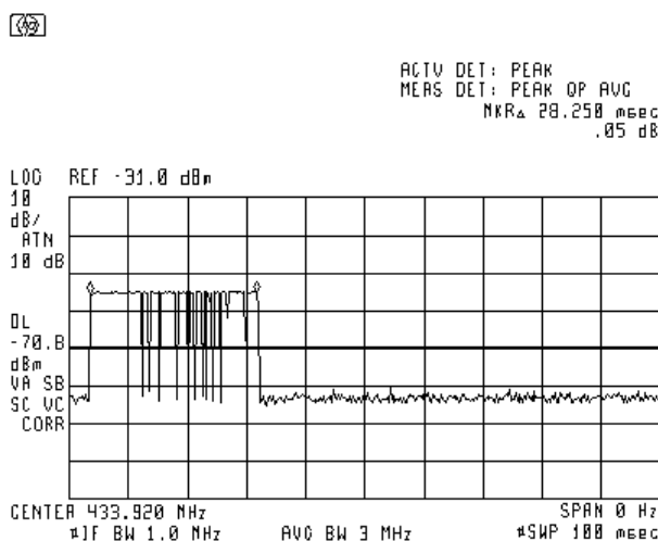
Plot 7.2.9 Transmission period
