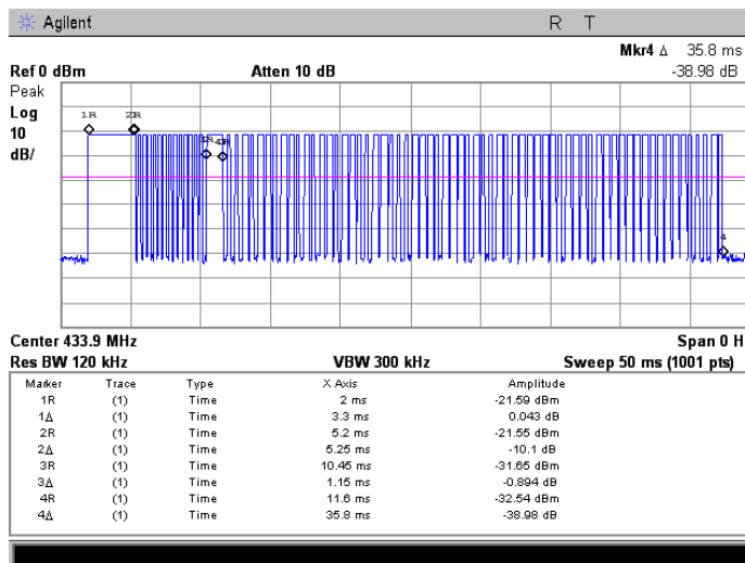
Plot 7.1.3 Polling / supervision transmission duration
