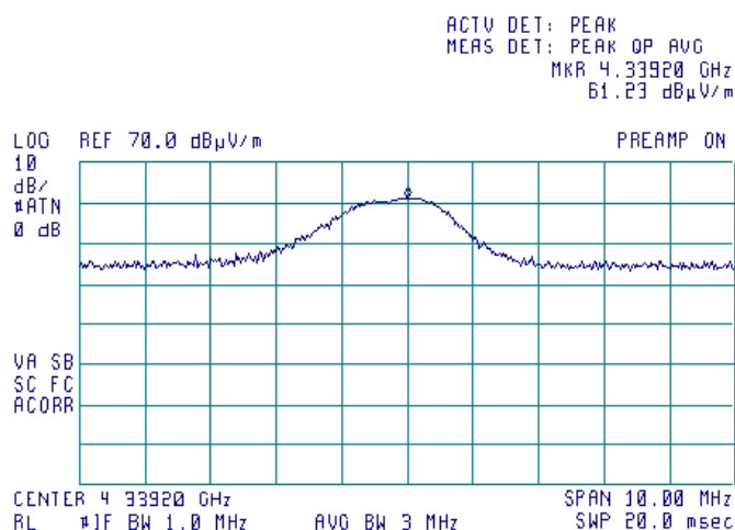
Plot 7.2.24 Radiated emission measurements at the tenth harmonic frequency
