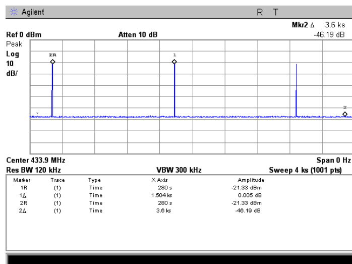
Plot 7.1.4 Total duration of polling / supervision transmission
