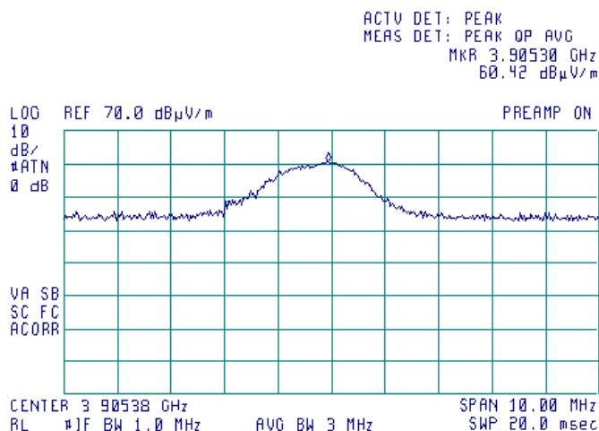
Plot 7.2.22 Radiated emission measurements at the ninth harmonic frequency
