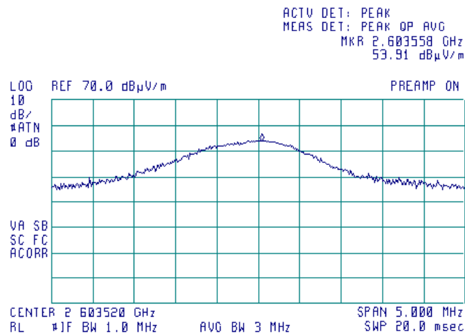
Plot 7.2.16 Radiated emission measurements at the sixth harmonic frequency
