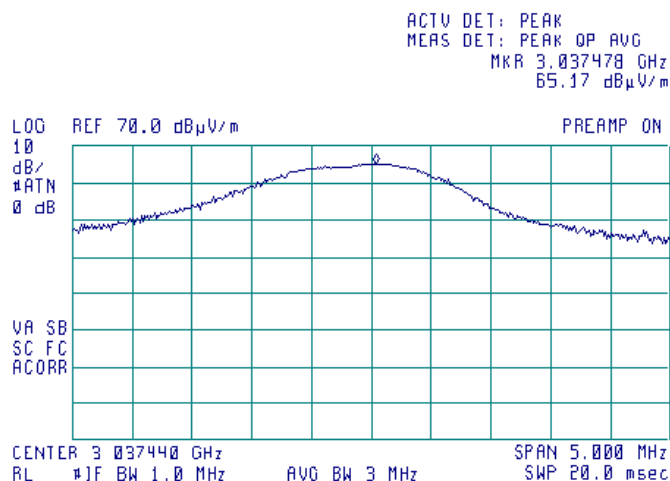
Plot 7.2.18 Radiated emission measurements at the seventh harmonic frequency
