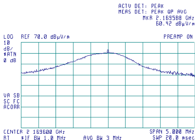
Plot 7.2.14 Radiated emission measurements at the fifth harmonic frequency
