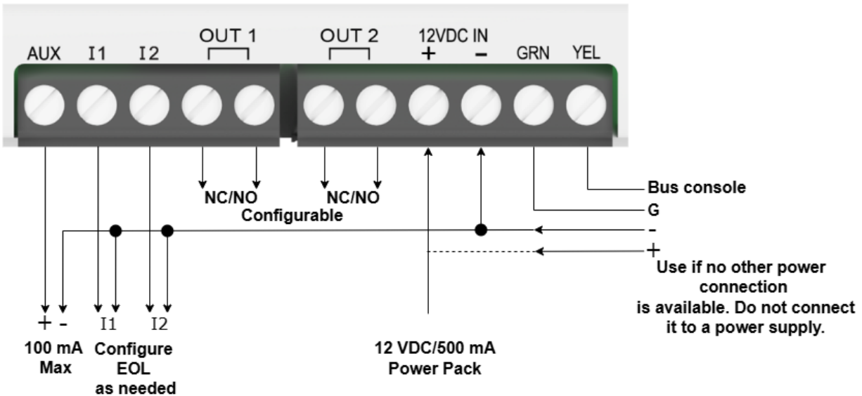
Fig 2 - Connection Diagram
