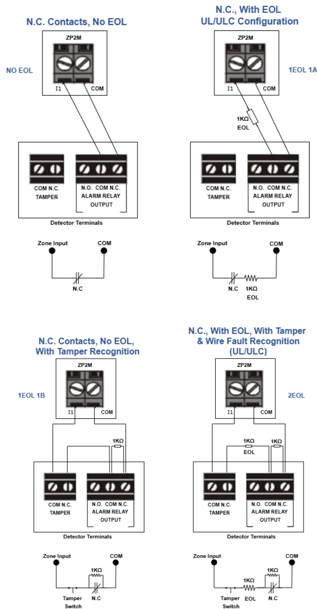
FIG-3 EOL Connection Options
