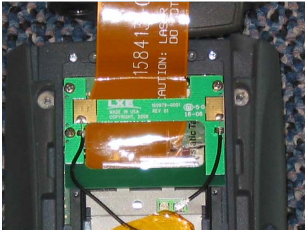
Main and Auxiliary Antennas
