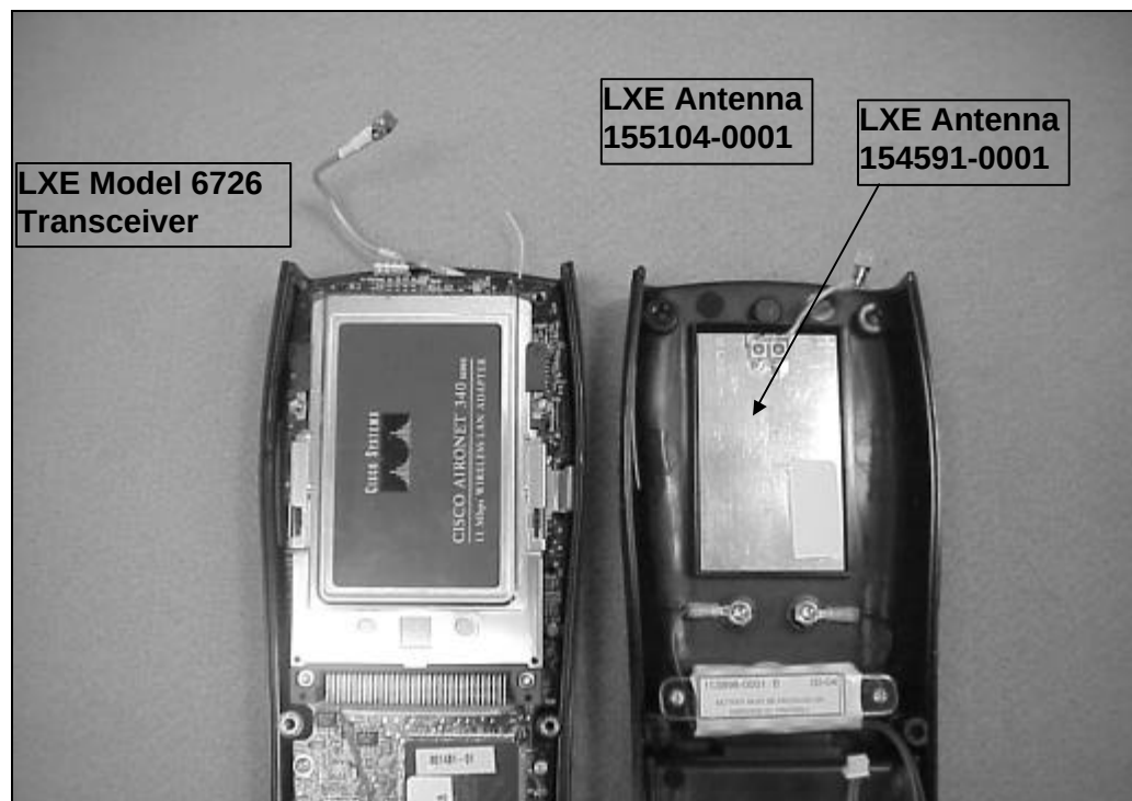
Figure 6: Internal view with back cover removed
