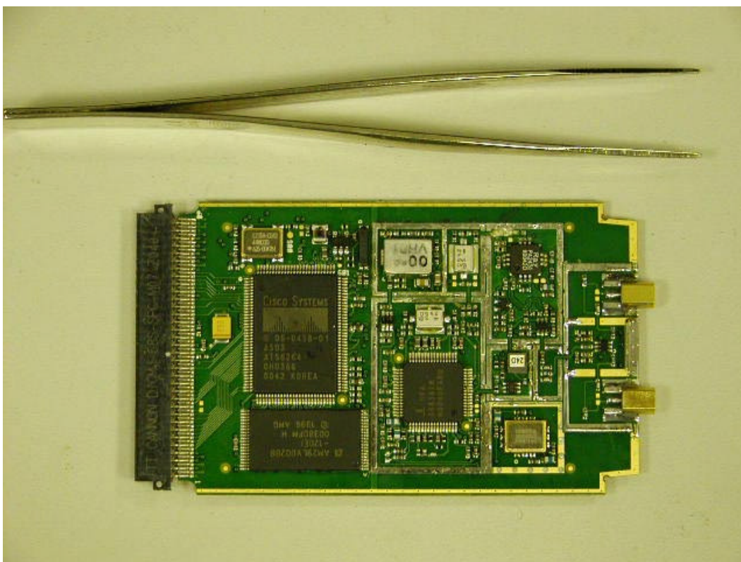
Internal view, topside, shields removed
