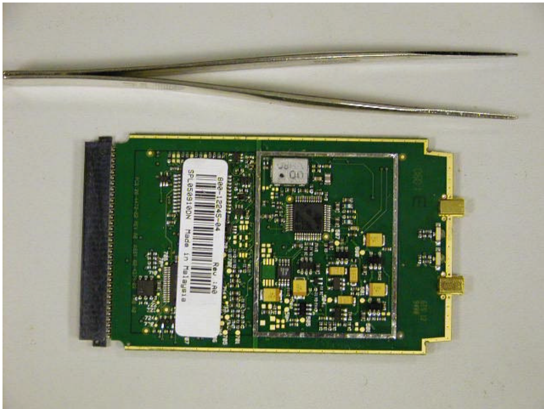
Internal view, bottom side with shields removed
