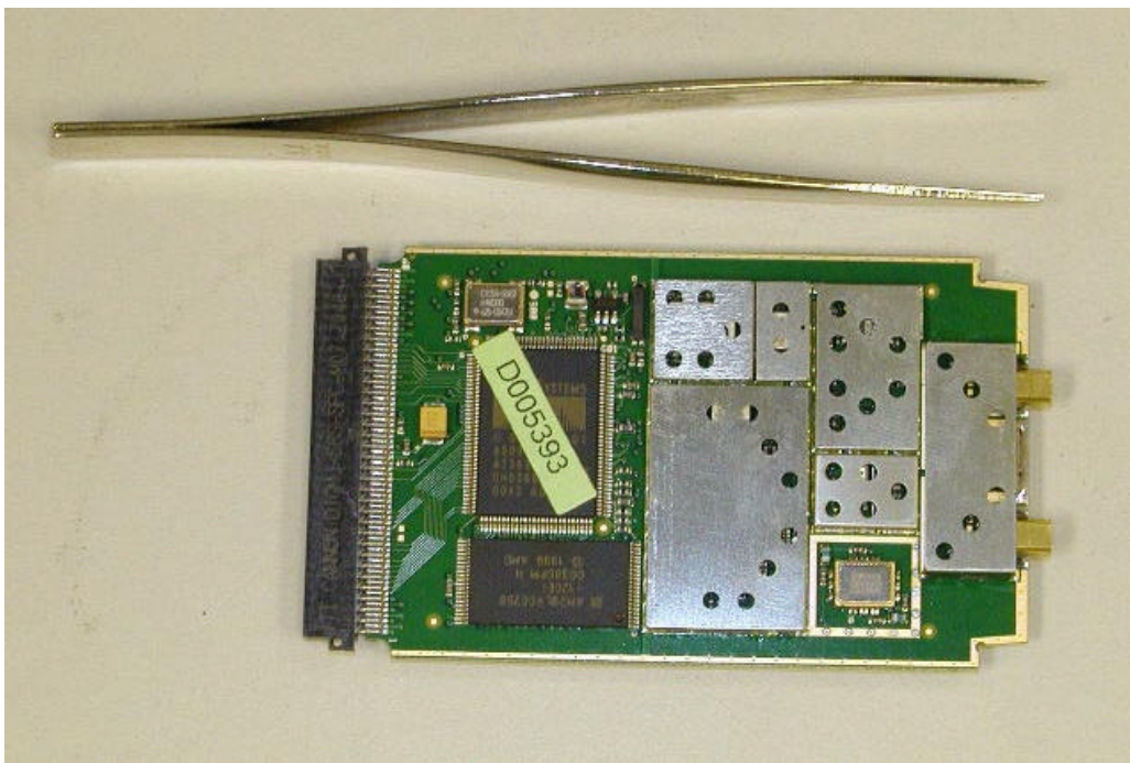
Internal view, topside with shields in place
