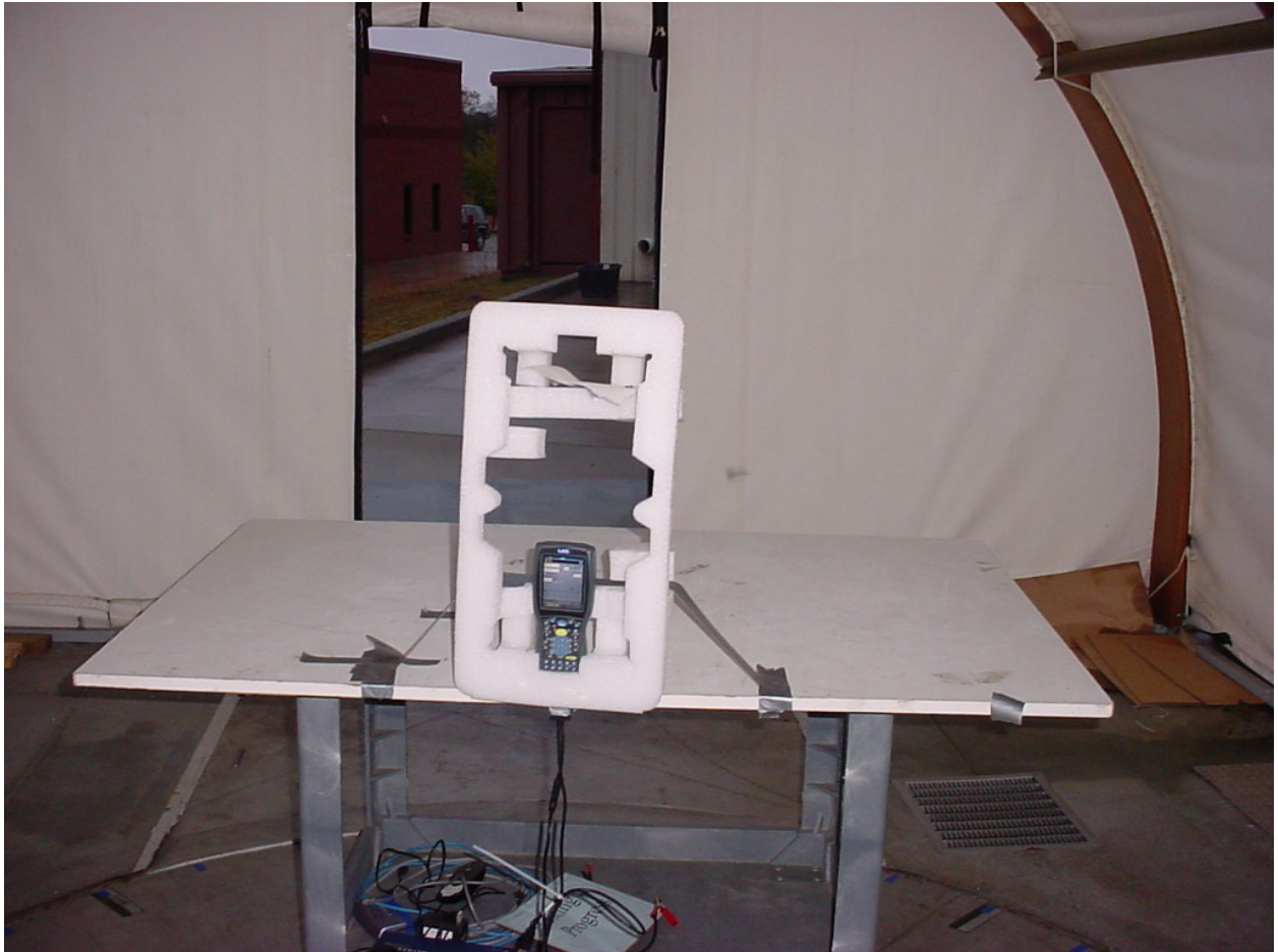
Figure 3: Radiated Emissions – Unintentional
