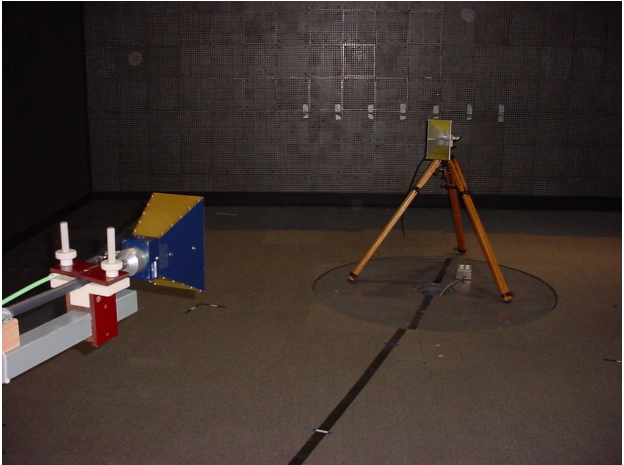
Figure 2: Radiated Emissions – Substitution
