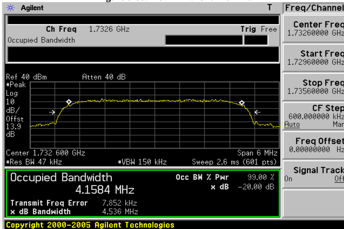
Figure 9-86: HSDPA IV Channel Mid
