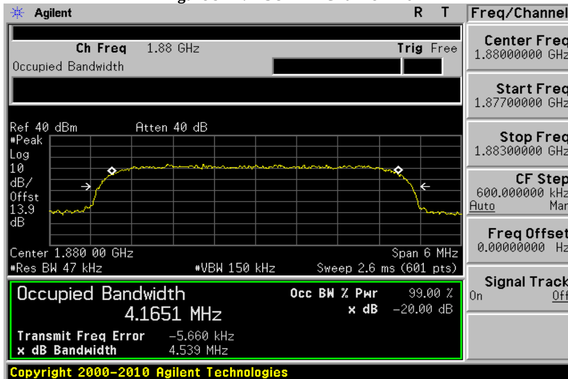
Figure 9-74: HSUPA II Channel Mid
