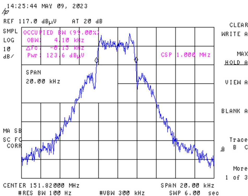
Figure 3. Bandwidth Measurement
