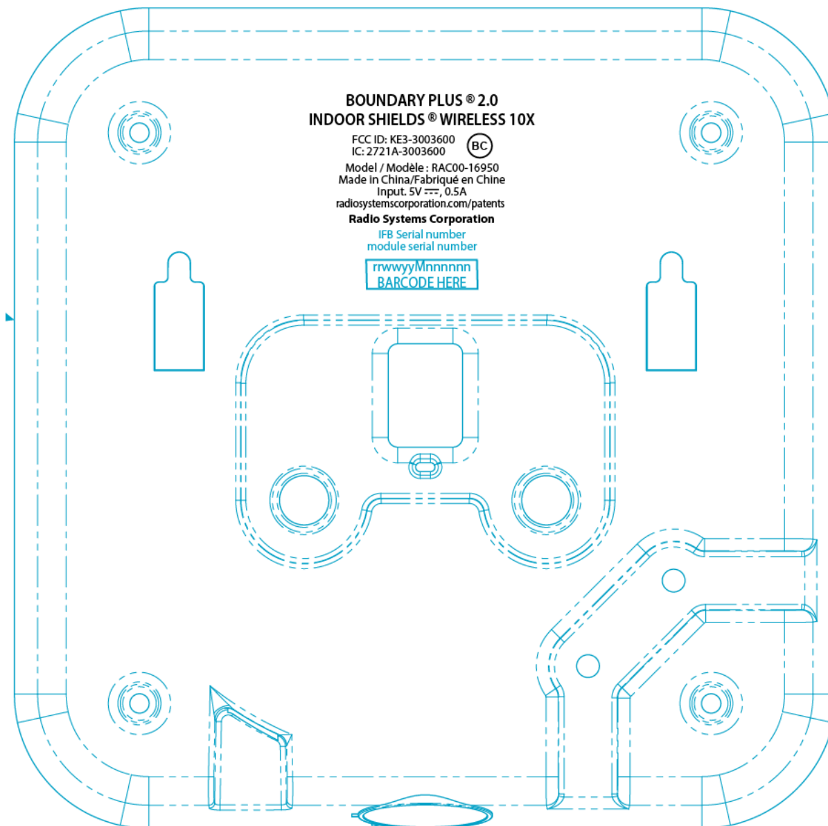
Figure 1. RAC00-16950 Sample Label and Location (Bottom of EUT)
