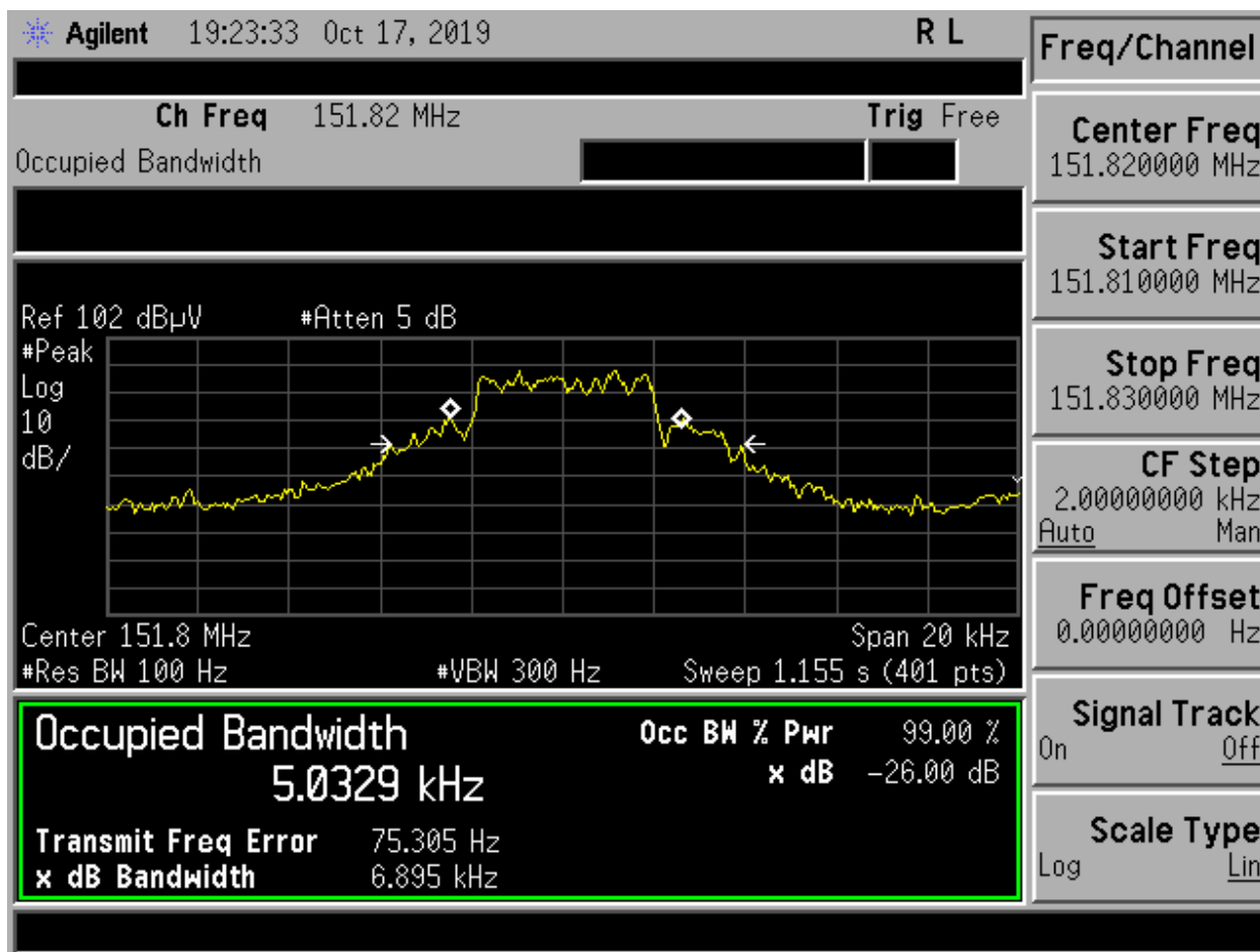
Figure 3. Bandwidth Measurement
