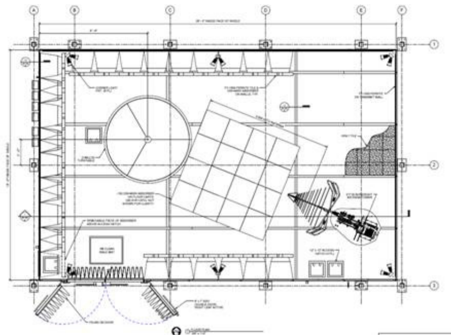
Figure 1. Radiated Emissions Disturbance Measurement Facility Diagram
