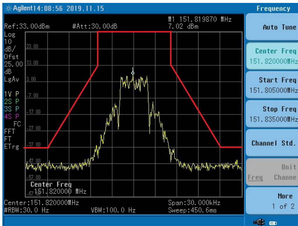
Figure 4. Emissions Mask
