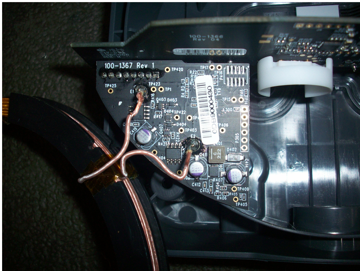
Figure 5. All Models, Top of PCB Component Side, 2 of 2
