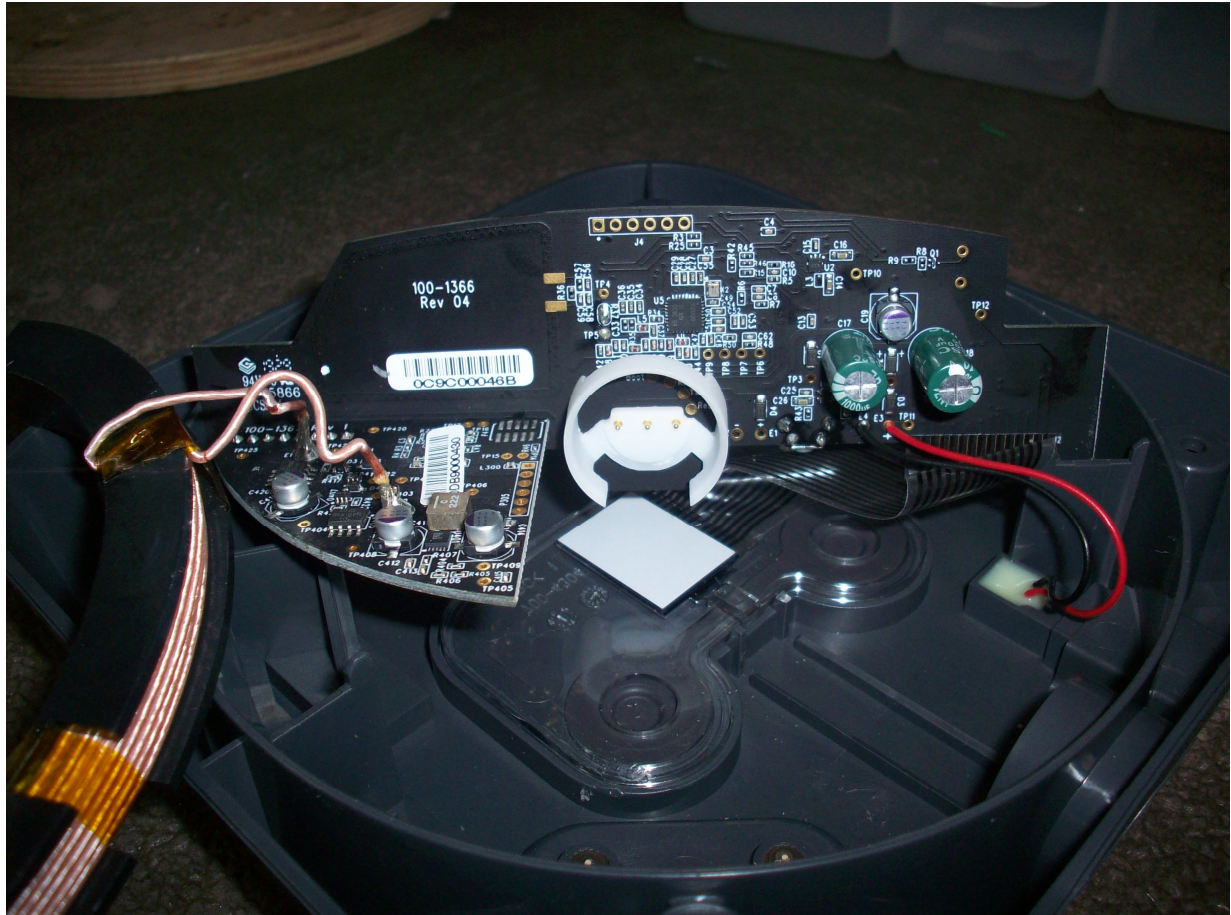
Figure 4. All Models, Top of PCB Component Side, 1 of 2
