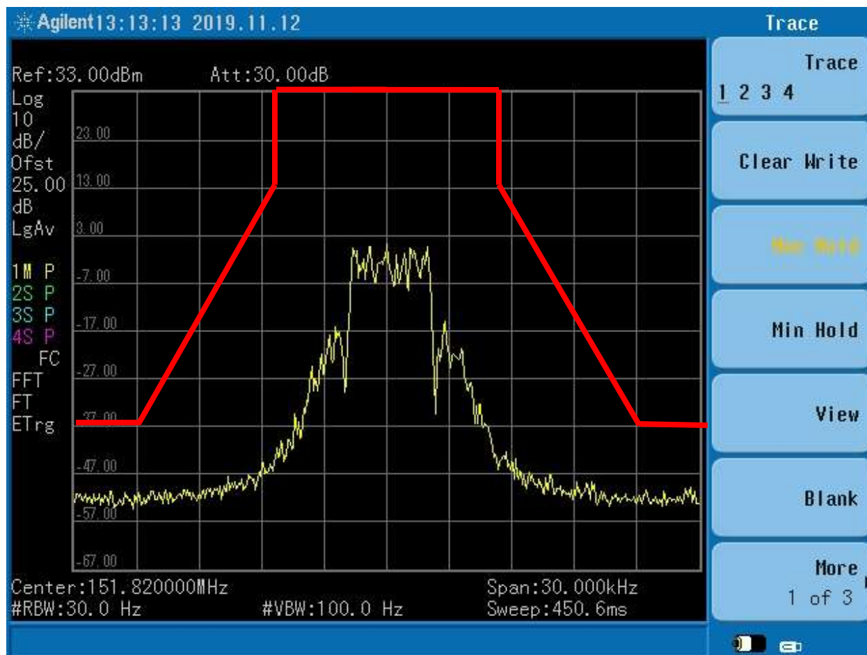
Figure 4. Emissions Mask
