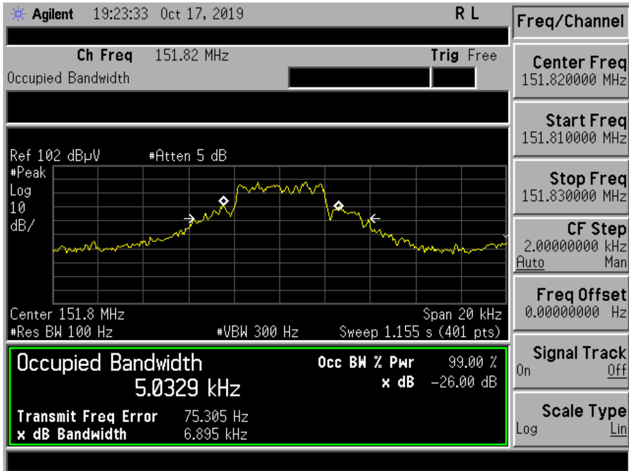
Figure 3. Bandwidth Measurement
