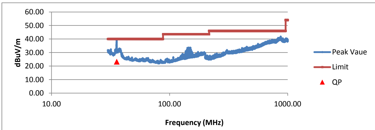
Figure 4. Radiated Emissions Graphical Data, 30 - 1000 MHz – Vertical
