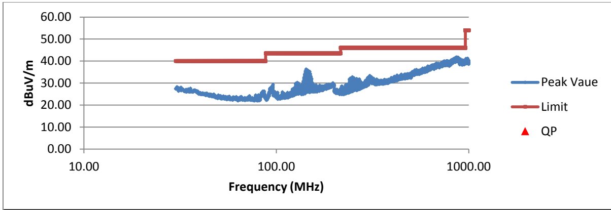
Figure 3. Radiated Emissions Graphical Data, 30 - 1000 MHz – Horizontal
