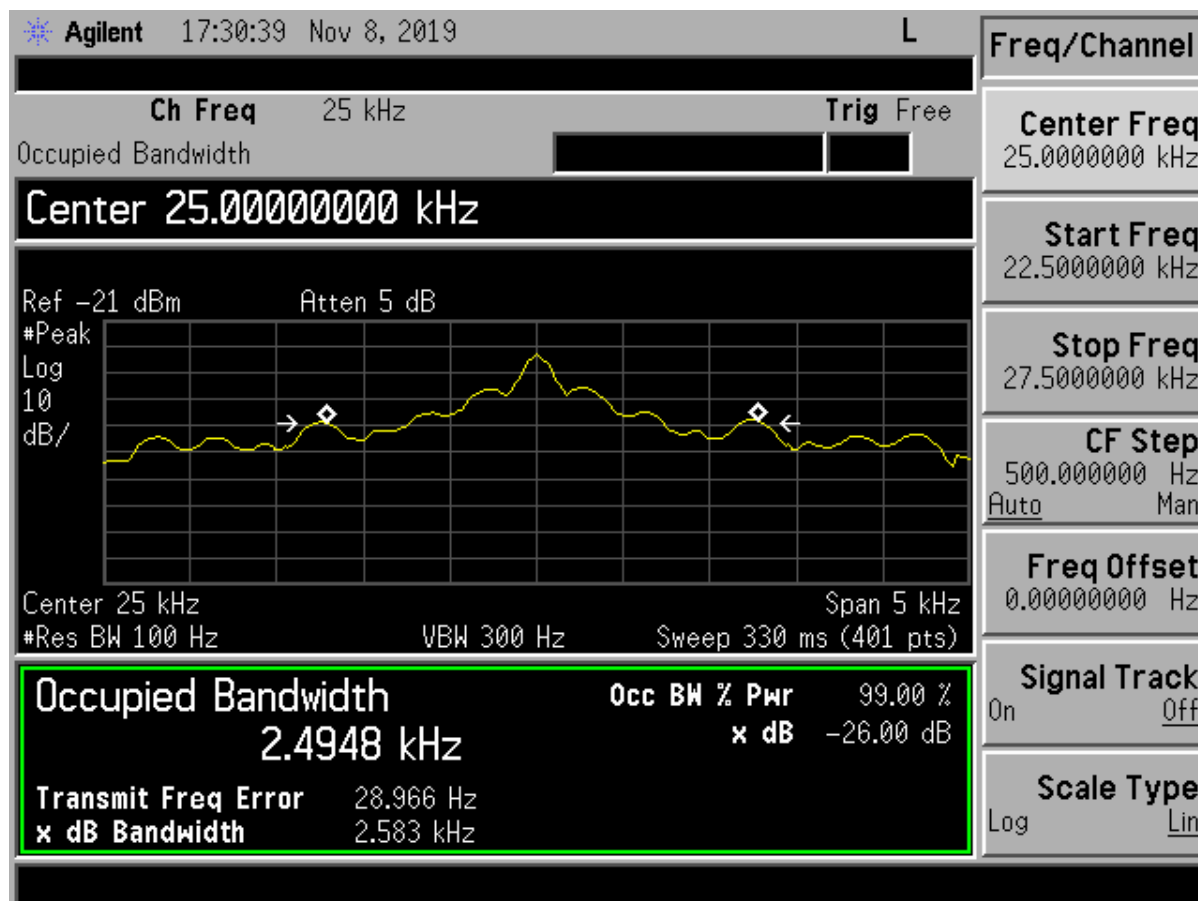
Figure 2. 99% Bandwidth
