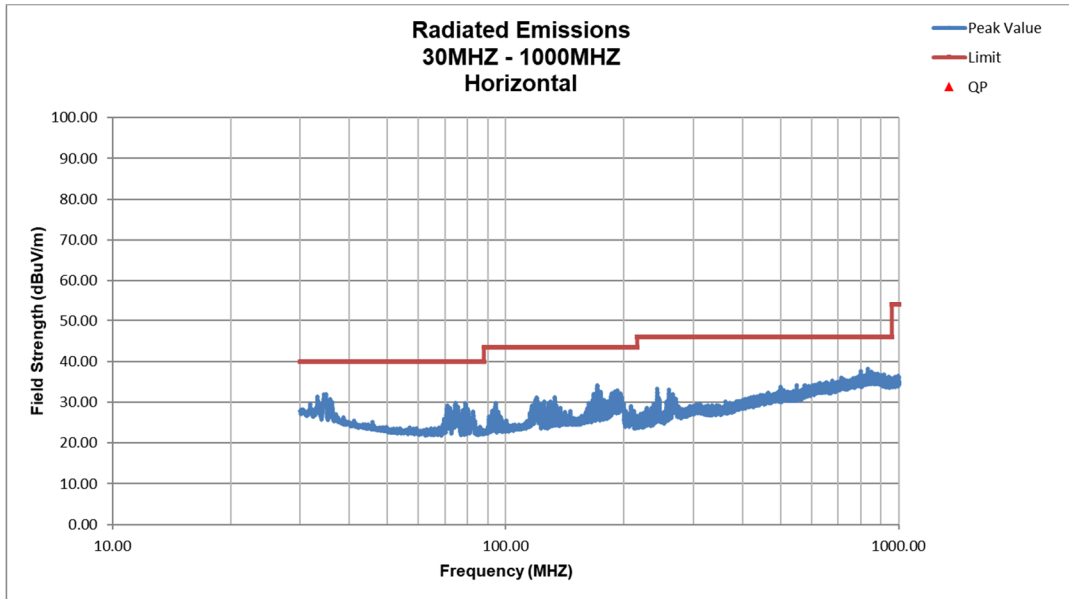
Figure 4. Radiated Emissions, Horizontal 30MHz – 1000MHz
