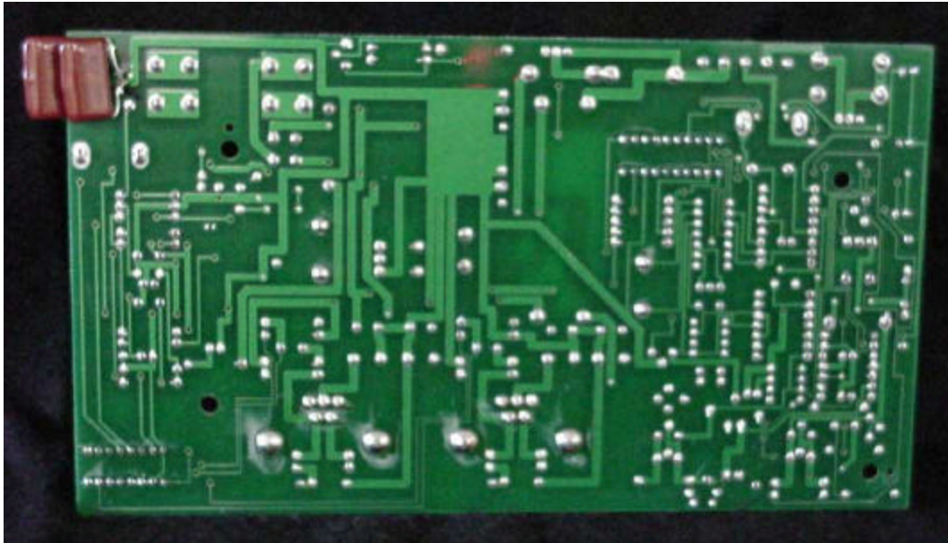
Photo 7. Main Board of EUT, Solder Side
