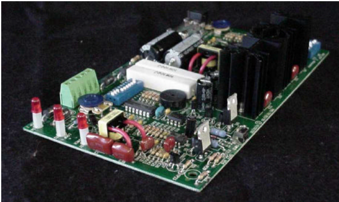
Photo 6. Main Board of EUT, PCB Side
