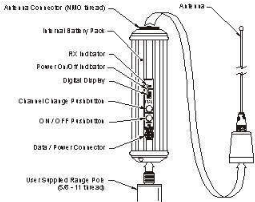
Figure 6 - PDL Rover
