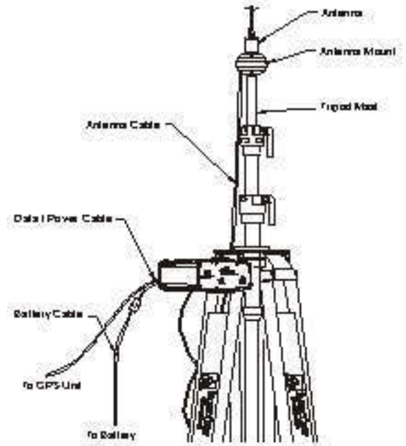
Figure 3 - PDL High Power Base System Setup
