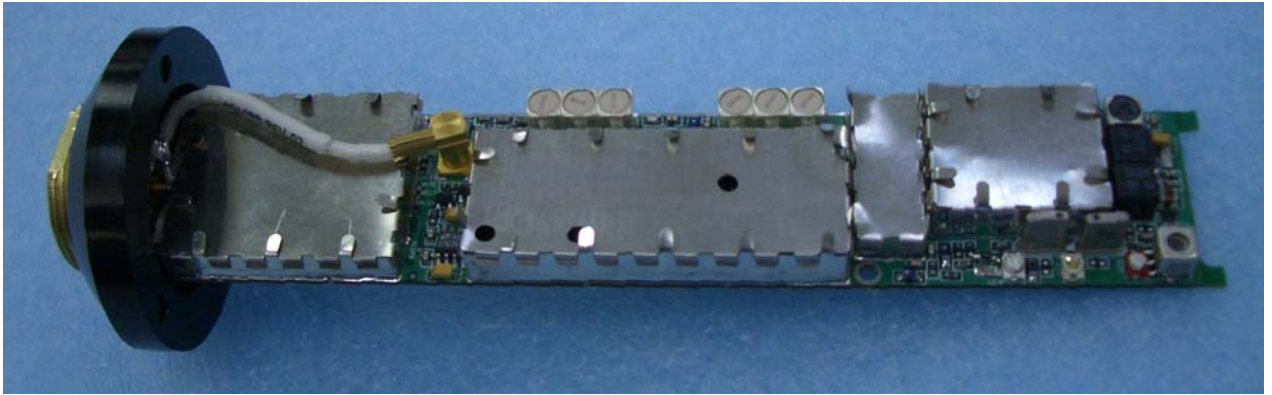
EUT – Radio PCB Top View with Antenna Connector
