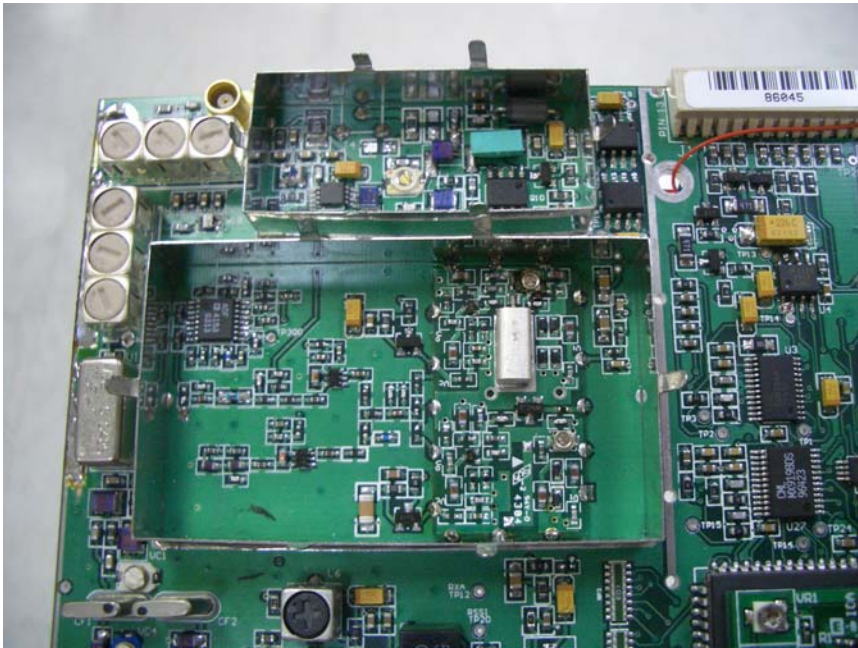
EUT – VCO Board
