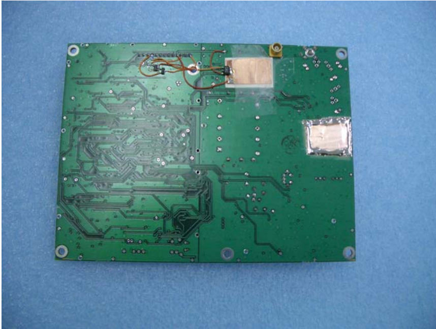
EUT – RF PCB Bottom View
