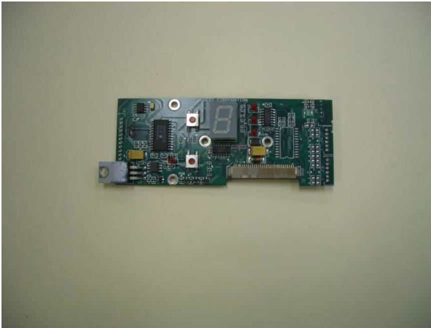
EUT – I/O Front Panel PCB Top View
