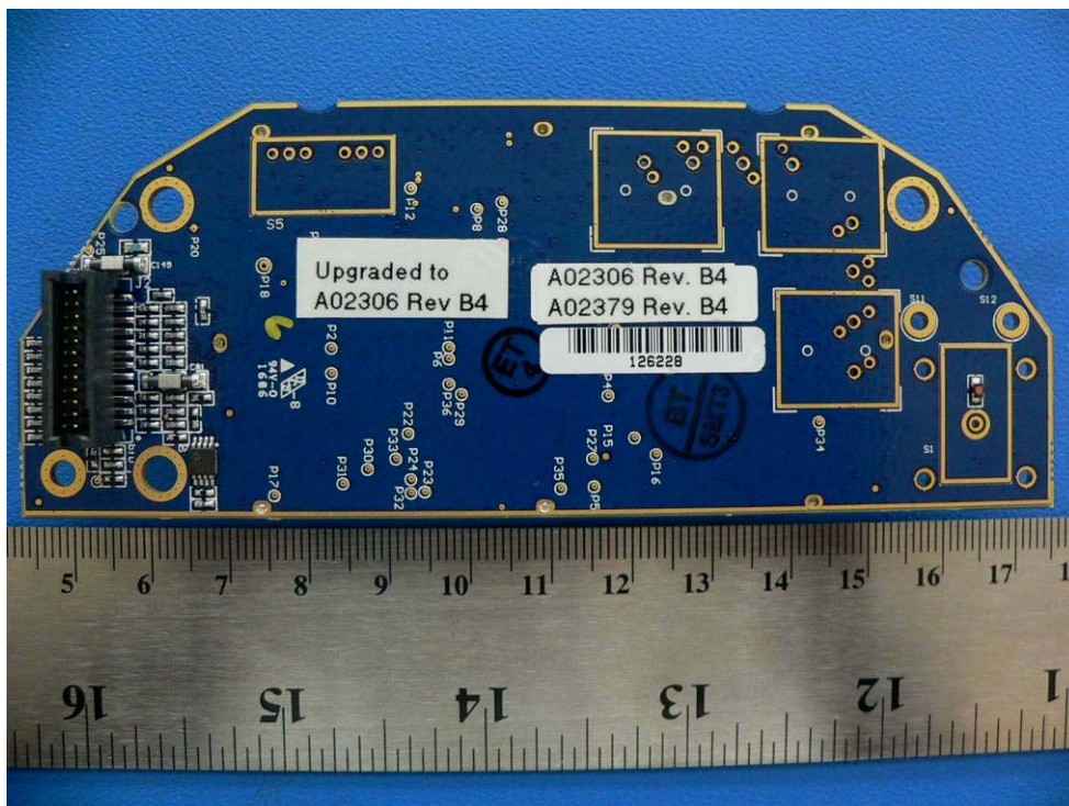
EUT components view 1 without shielding
