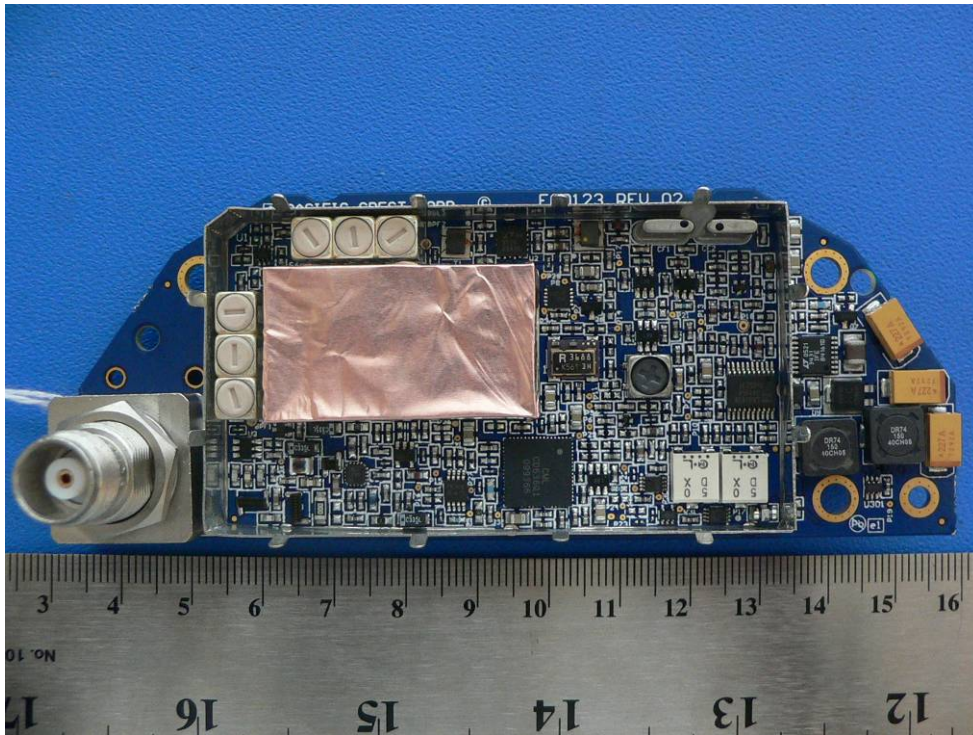
EUT components view 2 without shielding 2
