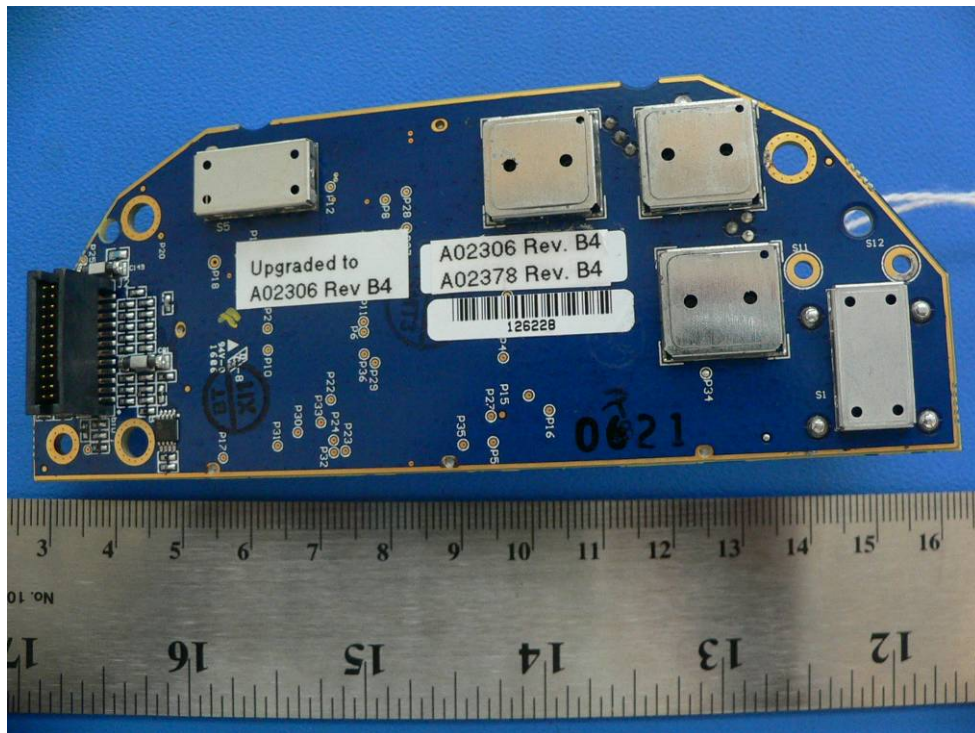
EUT components view 1 with shielding
