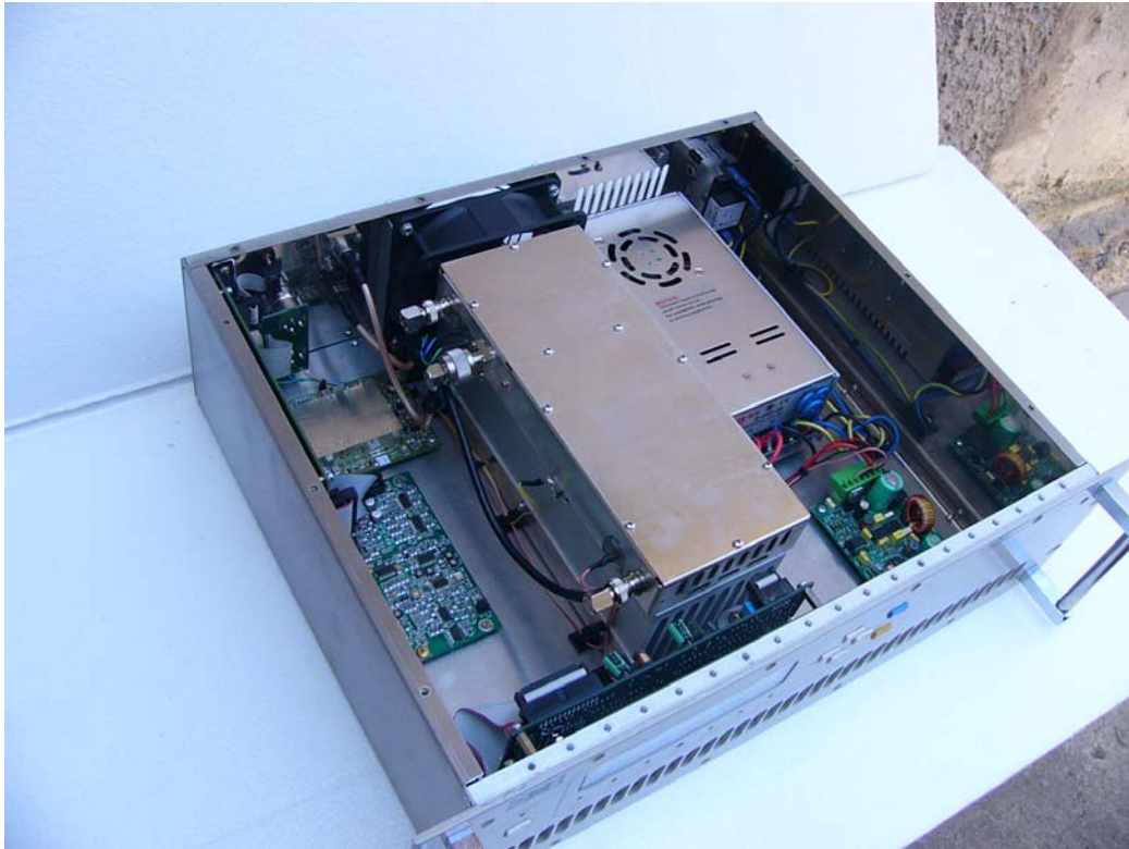
Top from left without main cover
