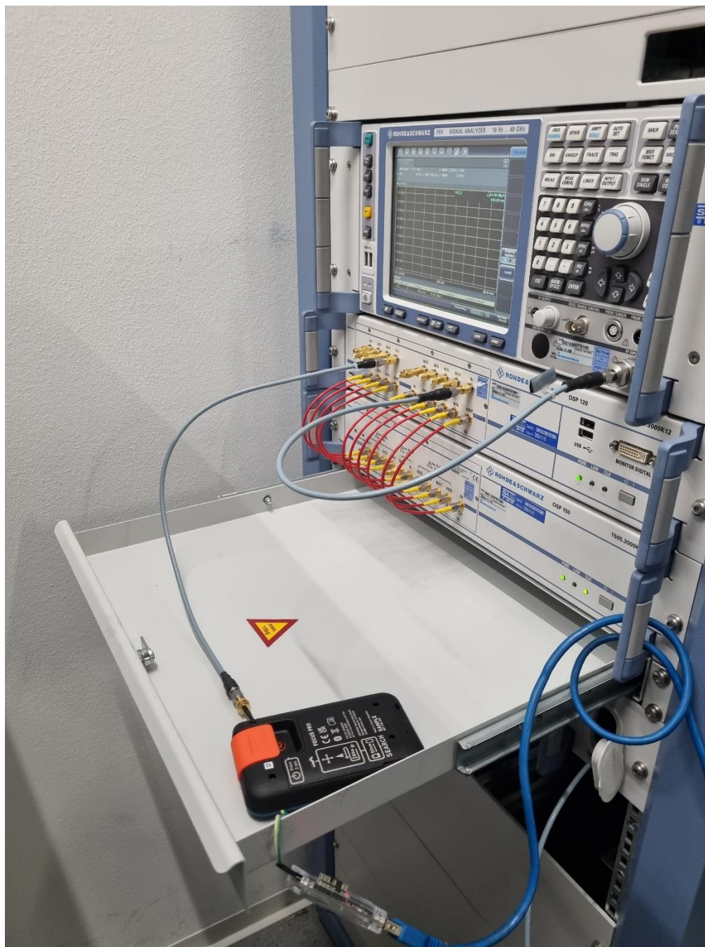
Figure 5: BLE Conducted measurements
