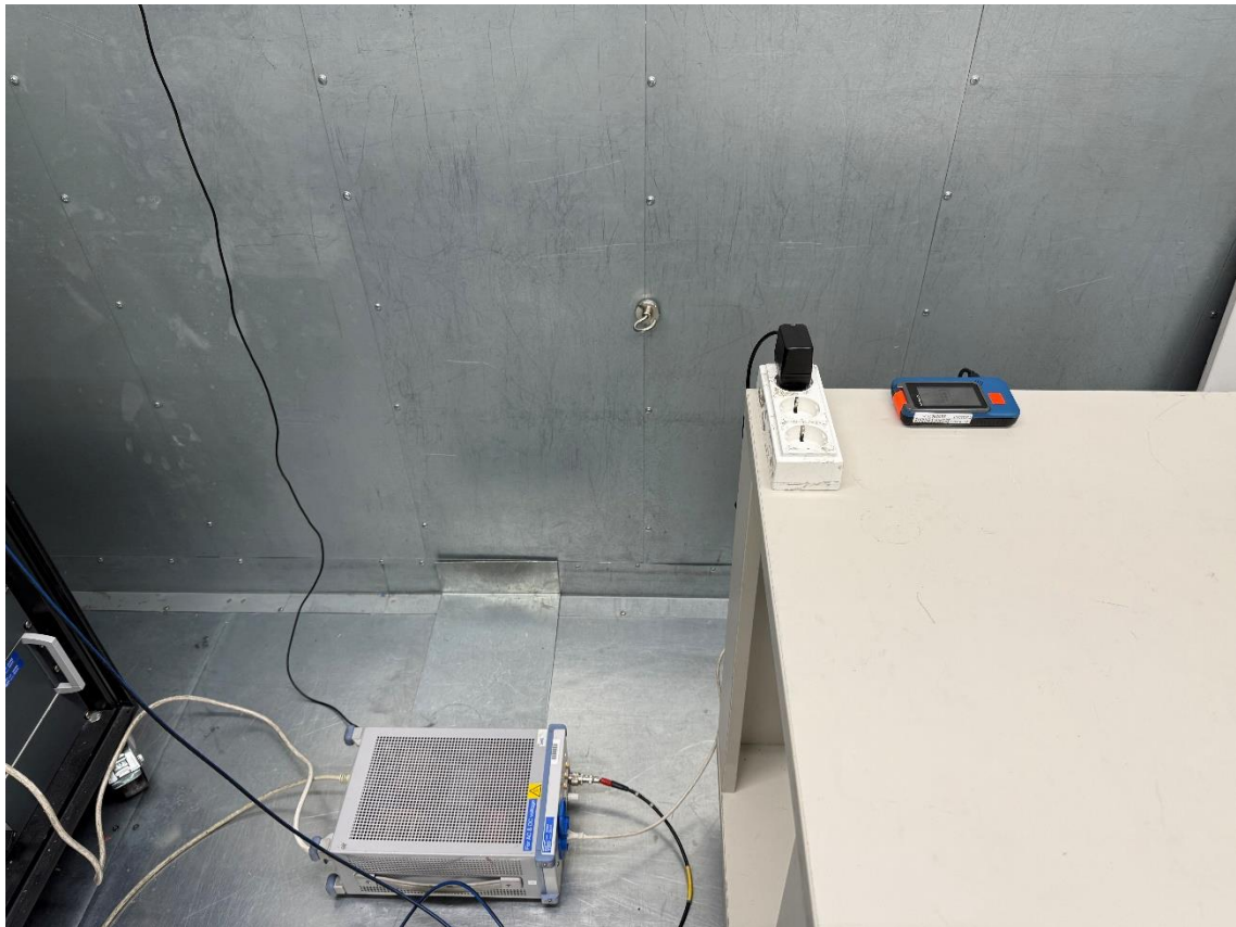
Figure 1: AC conducted emissions
