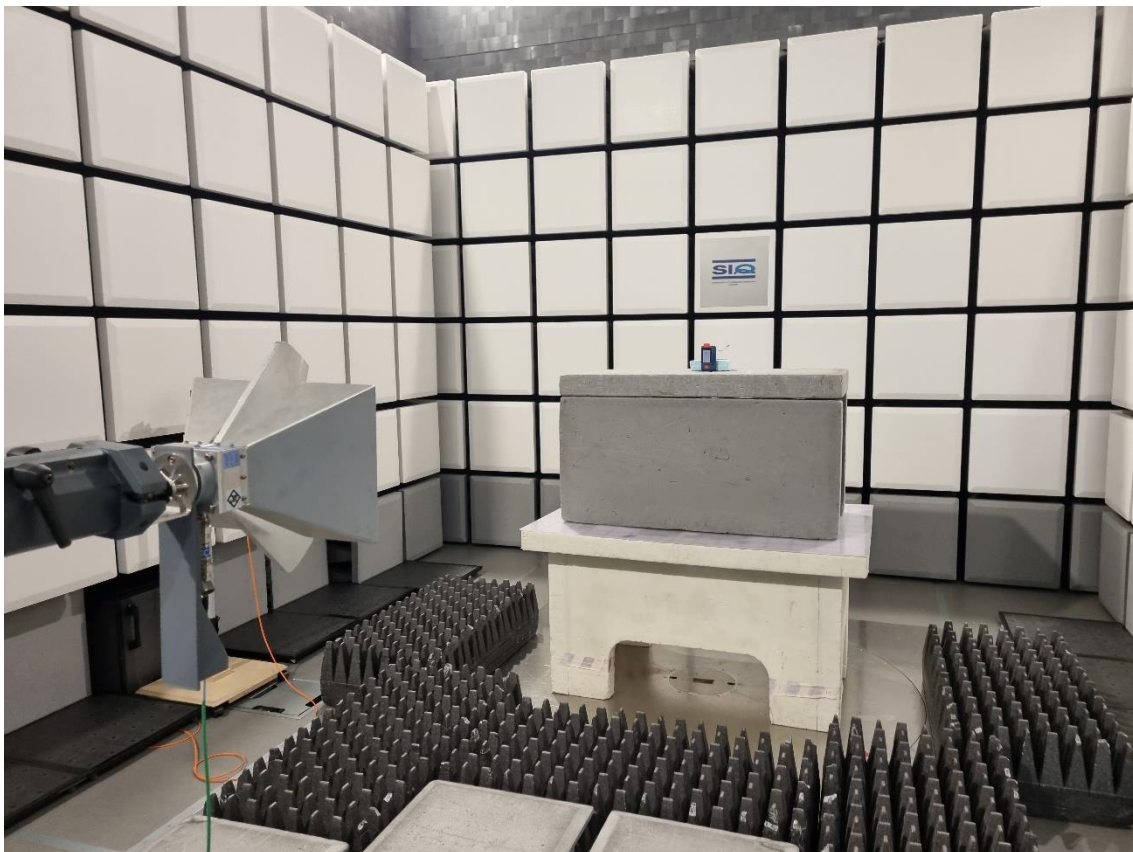
Figure 4: Radiated emissions 1 GHz – 18 GHz
