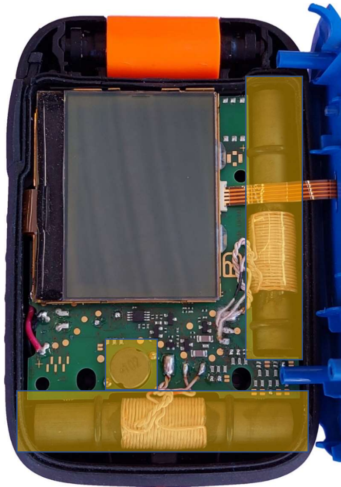
Internals of device with marked Antennas (Yellow)
