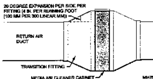
Fig. 11. Duct size changed gradually to prevent turbulence.
