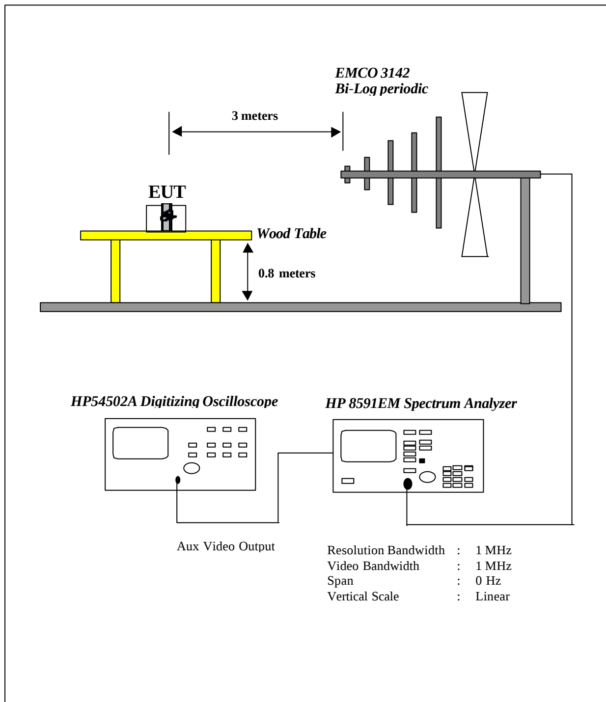
fig 1. Test Configuration of Duty Cycle Measurement
