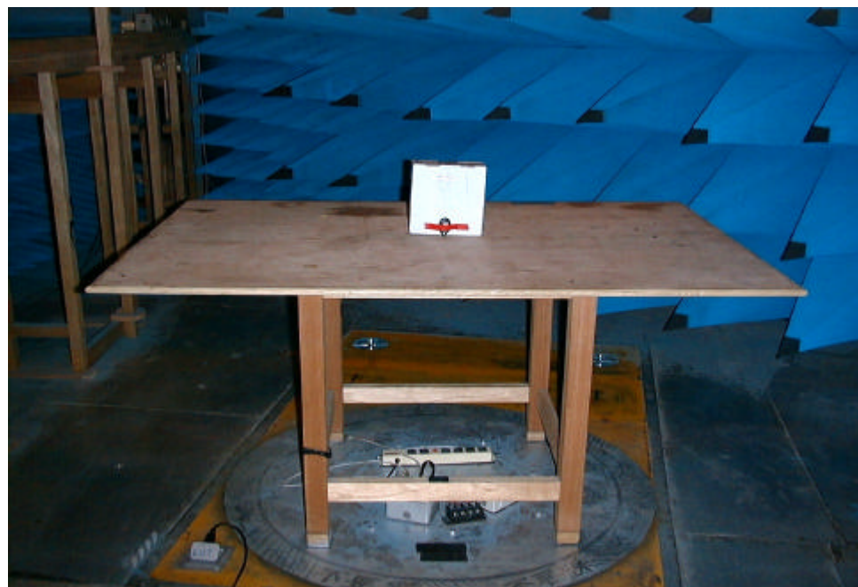
fig 2. Test Configuration of the Radiated Emissions (Back View)
