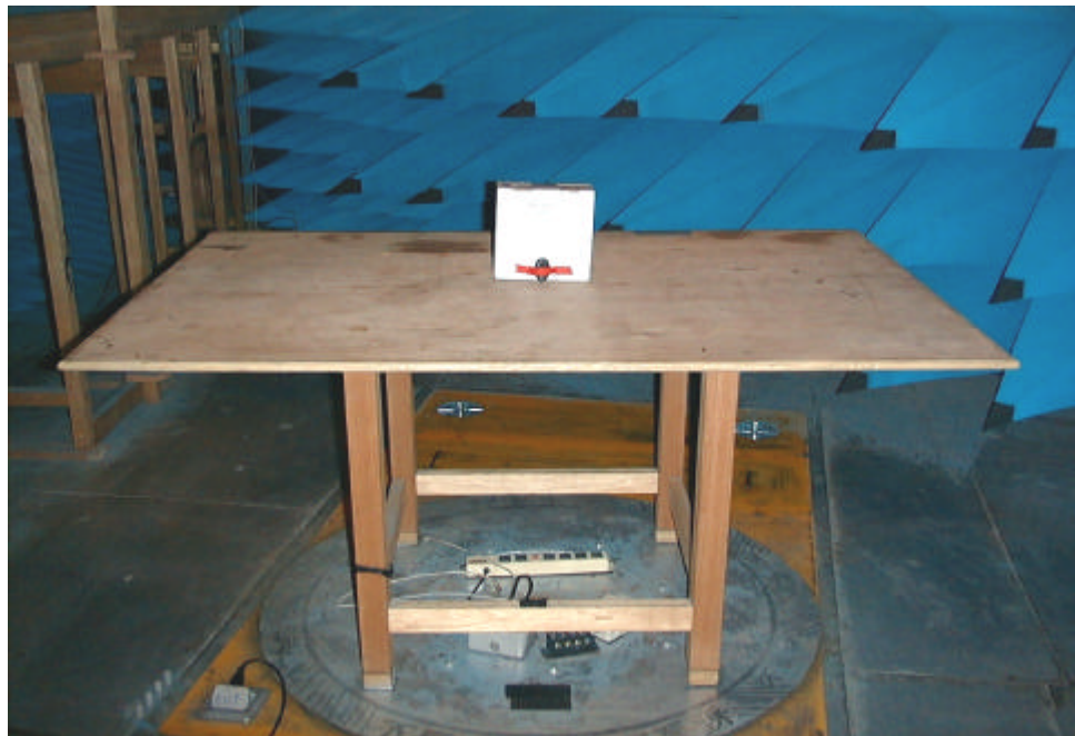
fig 1. Test Configuration of the Radiated Emissions (Front View)
