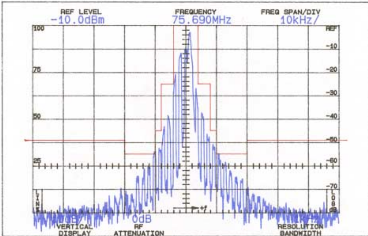
FIGURE 1 OCCUPIED BANDWIDTH
